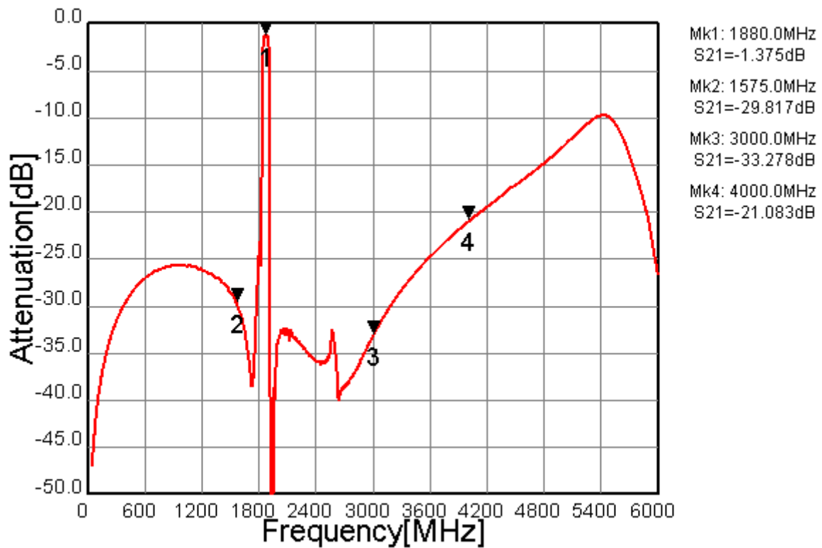
Fig.4 Wide-band Characteristics
