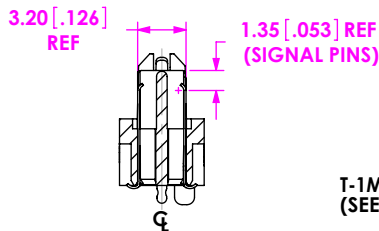
SECTION "N"-"N"
