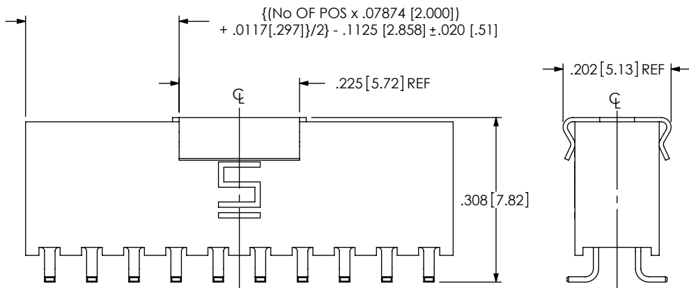
FIG 6 -P: PICK & PLACE PAD (4 POS MIN) SQW-110-01-XXX-D-VS-P SHOWN (DIFFERENT AS SHOWN, OTHERWISE SAME AS FIG 1)
