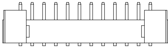
FIG 2 -ES: END SHROUDS FTMH-112-02-X-DV-ES SHOWN (DIFFERENT AS SHOWN, OTHERWISE SAME AS FIG 1)
