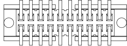
FIG 4 -DV-SA OPTION (SEE NOTES 6 & 7) FTS-106-02-XX-DV-SA SHOWN (DIFFERENT AS SHOWN, OTHERWISE SAME AS FIG 1) NOTE: 4 POSITIONS MUST BE ADDED TO PART CALLOUT TO ACHIEVE DIMS
