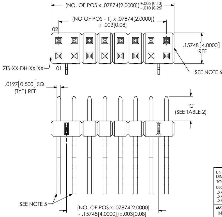
FIG 1 MMT-108-01-X-DH-LC SHOWN
