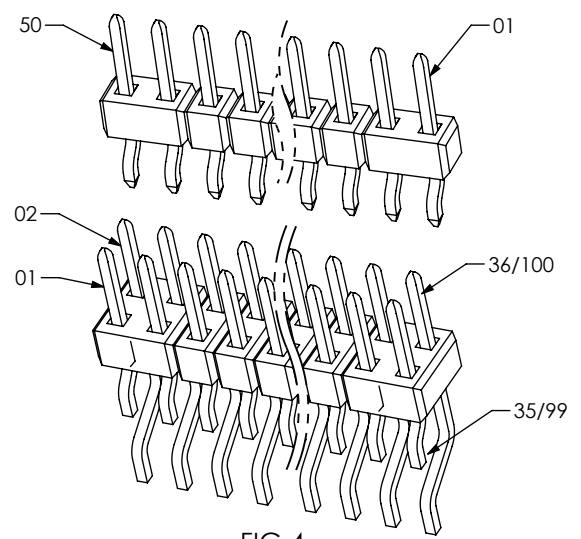
FIG 4 POLARIZATION VIEW
