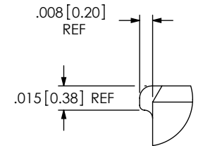
DETAIL 'E' SCALE 12:1
