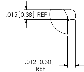
DETAIL 'F' SCALE 12:1
