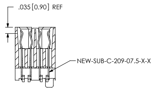
SECTION "F"-"F"
