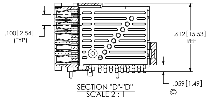
FIG 9 (SEAF-20-01-X-T0-X-RA-GP SHOWN) (SAME AS FIG 4 EXCEPT AS NOTED) (SOME DETAIL REMOVED FOR CLARITY)
