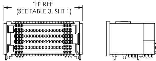
FIG 9 (SEAF-20-01-X-T0-X-RA SHOWN) (SAME AS FIG 4 EXCEPT AS NOTED) (SOME DETAIL REMOVED FOR CLARITY)
