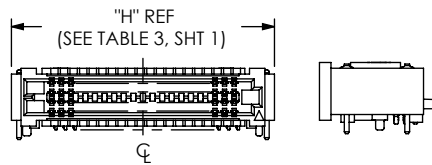
FIG 2 (SEAF-20-01-X-04-X-RA SHOWN) (SAME AS FIG 1 EXCEPT AS NOTED) (SOME DETAIL REMOVED FOR CLARITY)
