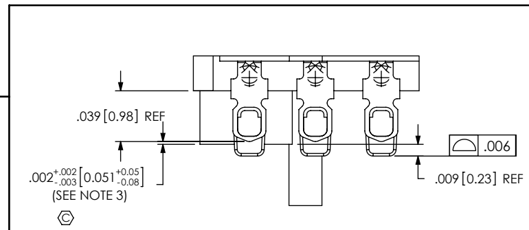
DETAIL 'F' SCALE 10:1
