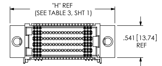
FIG 9 (SEAF-20-01-X-T0-X-RA-GP SHOWN) (SAME AS FIG 4 EXCEPT AS NOTED) (SOME DETAIL REMOVED FOR CLARITY)
