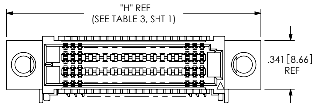
FIG 3 (SEAF-20-01-X-06-X-RA-GP) (SAME AS FIG 1 EXCEPT AS NOTED) (SOME DETAIL REMOVED FOR CLARITY)
