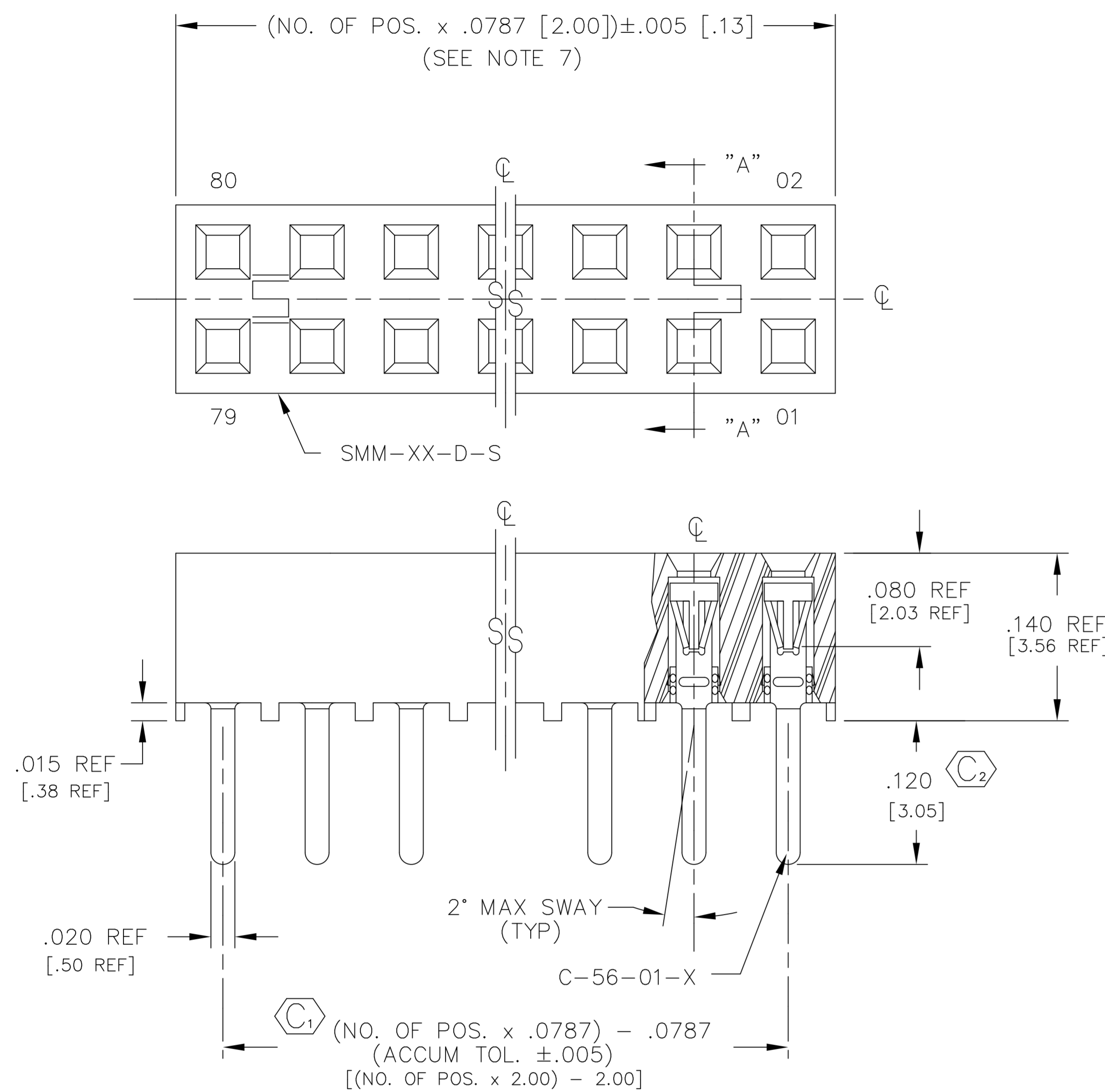
FIG. 1 -01: THROUGH HOLE
