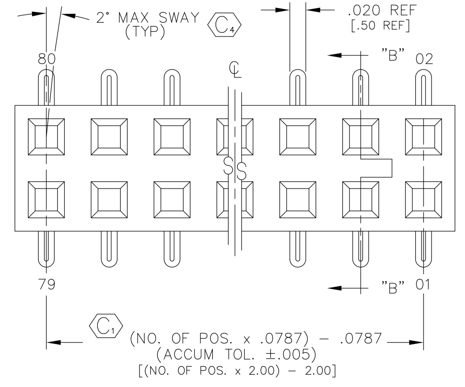
FIG. 2 -02: SURFACE MOUNT
