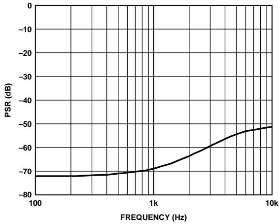
Figure 5. Typical Power Supply Rejection Ratio vs. Frequency
