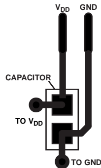
Figure 14. Recommended Power-Supply Bypass Capacitor Layout
