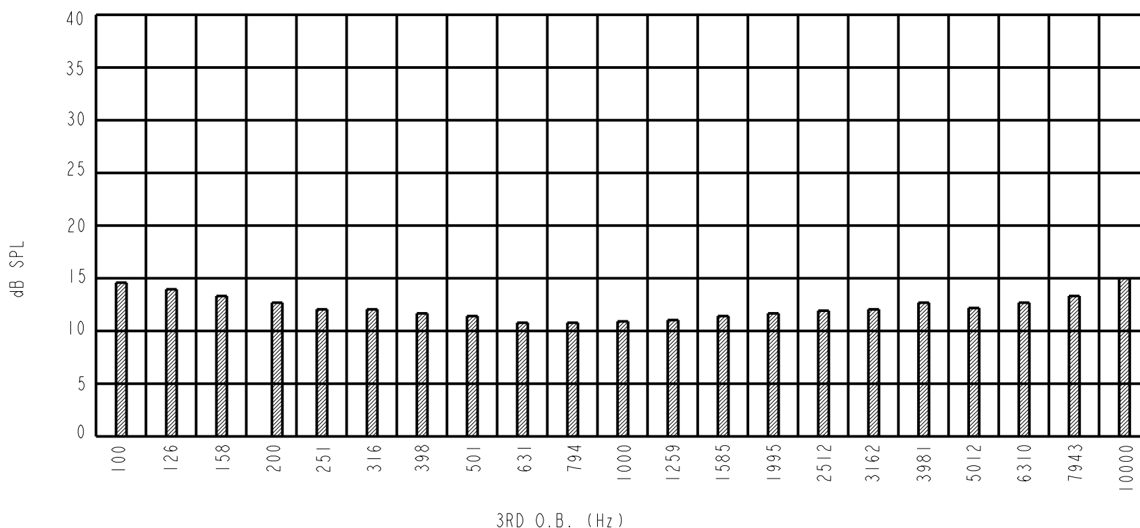
1/3RD OCTAVE BAND INPUT REFERRED NOISE - TYPICAL
