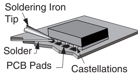
Figure 44: Soldering Technique
