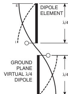
Figure 25: Dipole Antenna
