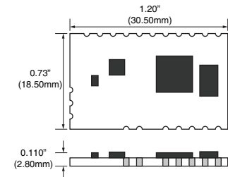
Figure 1: Package Dimensions
