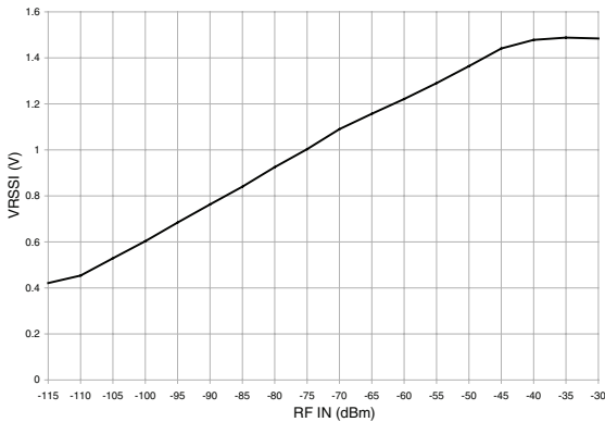
Figure 8: RSSI Curve
