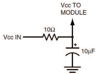
Figure 22: Supply Filter
