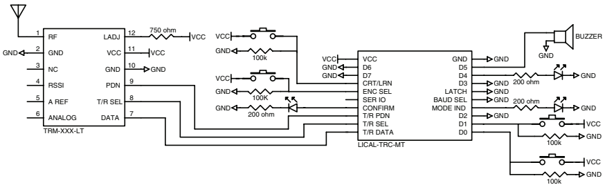
Figure 24: LT Transceiver and MT Transcoder
