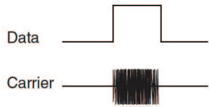
Figure 21: CPCA (AM) Modulation
