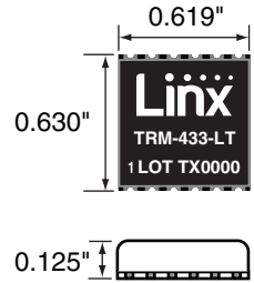
Figure 1: Package Dimensions
