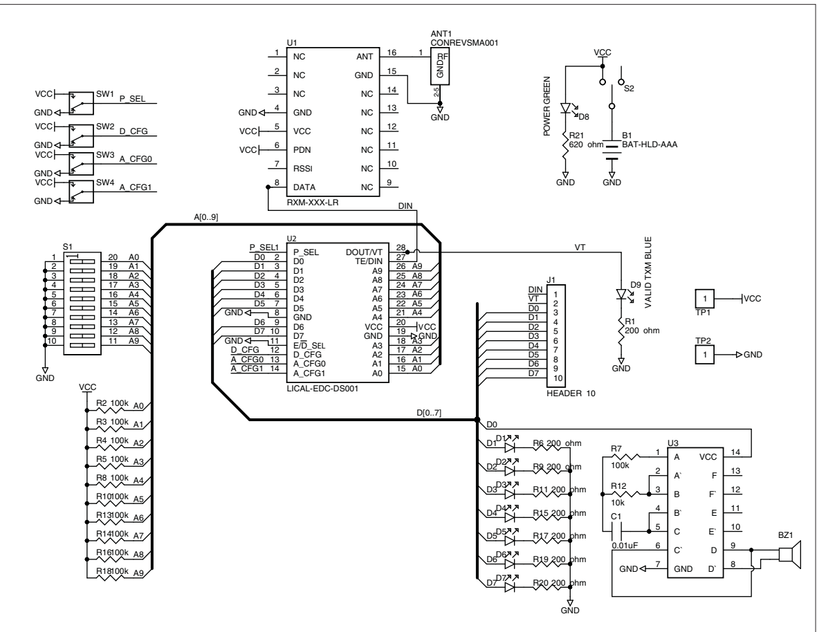
Figure 6: DS Series Decoder Board Schematic
