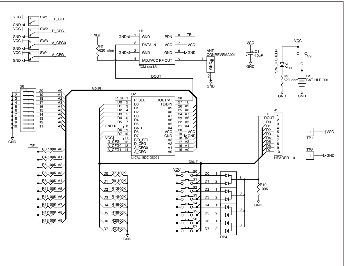
Figure 5: DS Series Encoder Board Schematic
