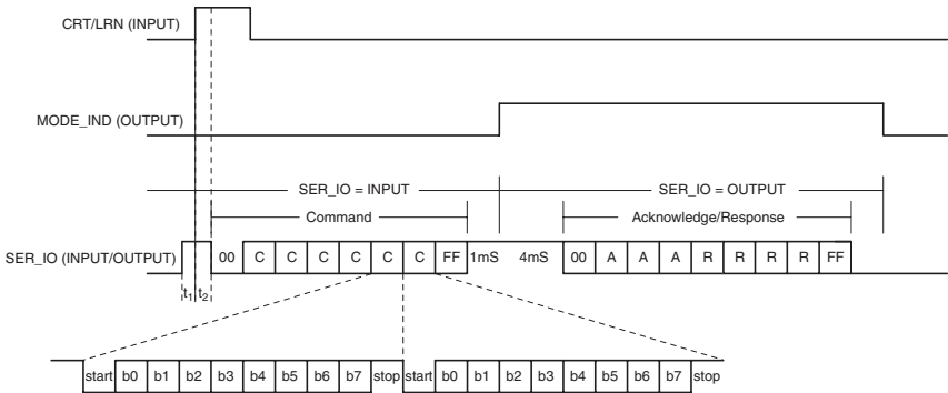
Figure 17: MT Series Transcoder Serial Programming
