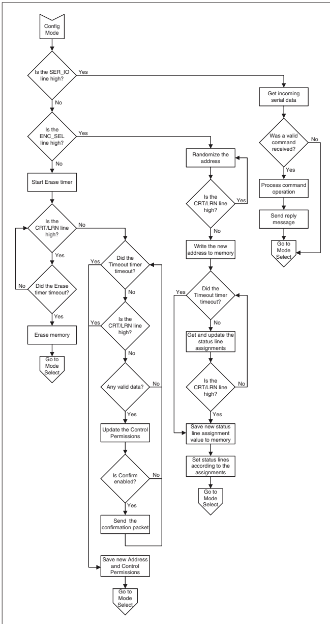
Figure 26: MT Series Transcoder Configure Flowchart
