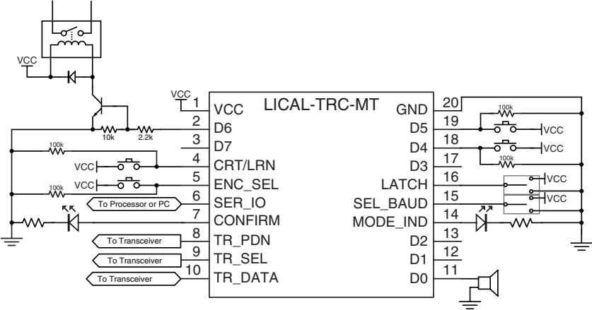
Figure 28: MT Series Transcoder Application Circuit
