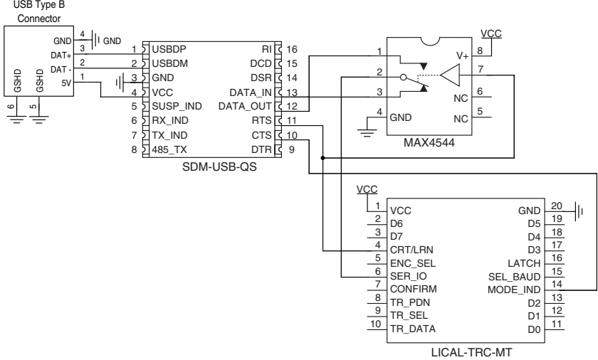
Figure 19: MT Series Transcoder Serial Interface to a PC
