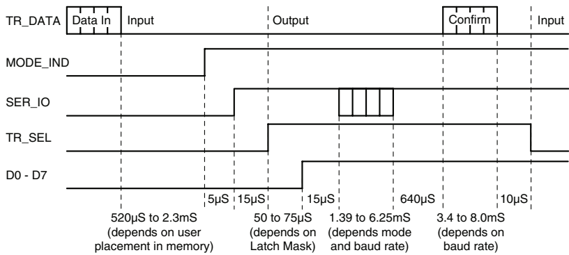
Figure 14: MT Series Receive Timings
