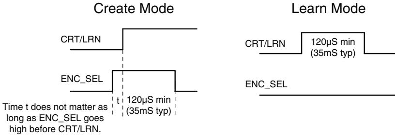
Figure 12: MT Series Mode Entry Timings
