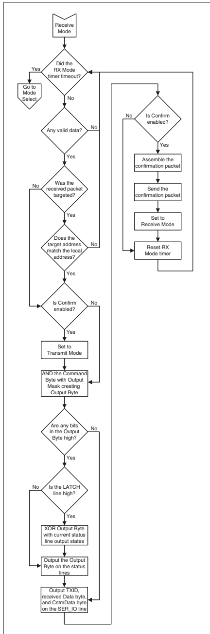
Figure 27: MT Series Transcoder Receive Flowchart
