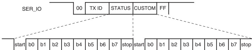
Figure 16: MT Series Transcoder Locked Access Serial Output
