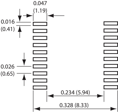
Figure 5: PCB Layout Dimensions
