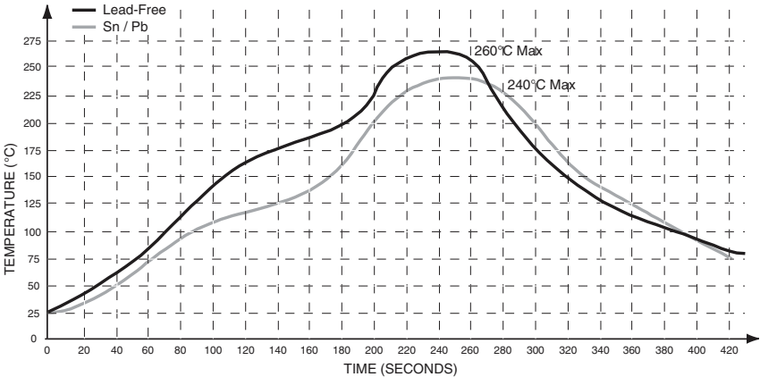
Figure 6: MT Series Reflow Profile
