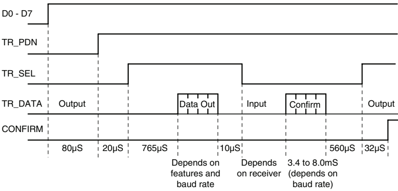
Figure 13: MT Series Transmit Timings
