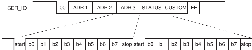
Figure 15: MT Series Transcoder Open Access Serial Output
