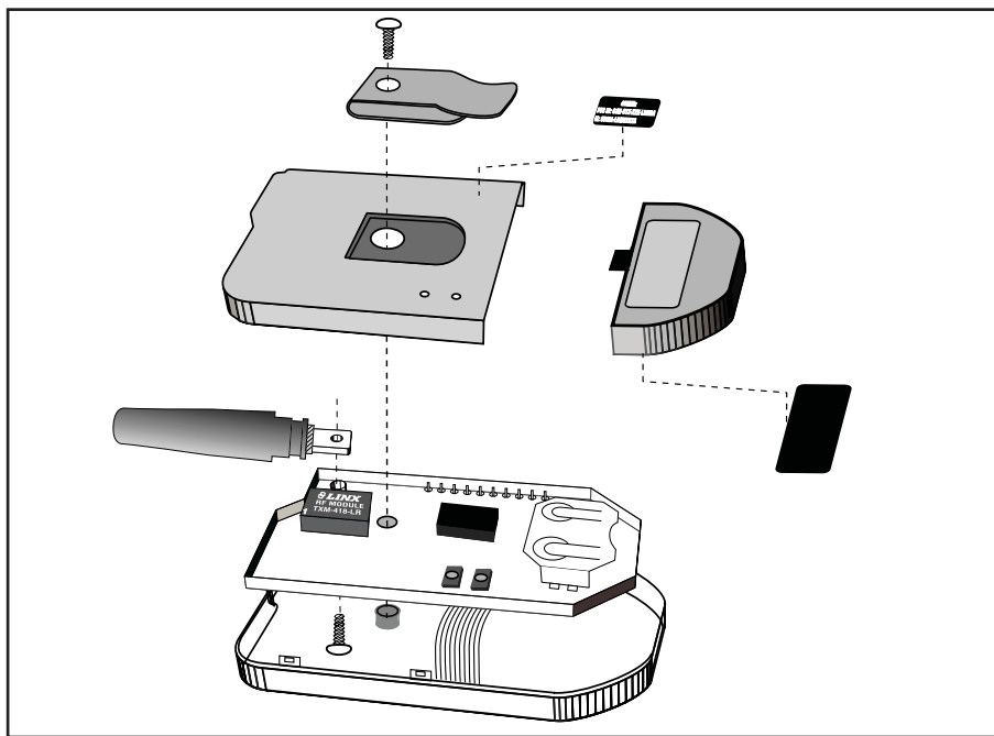
Figure 5: OTX-***-HH-LR8-MS Assembly
