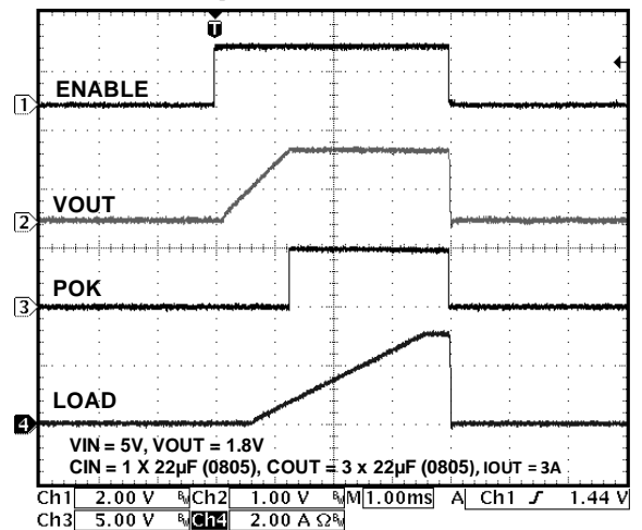
Startup Waveforms at 3A
