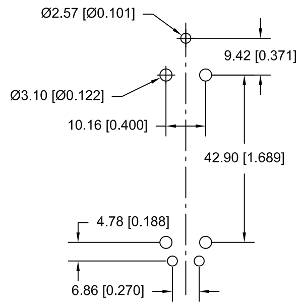
PCB LAYOUT
