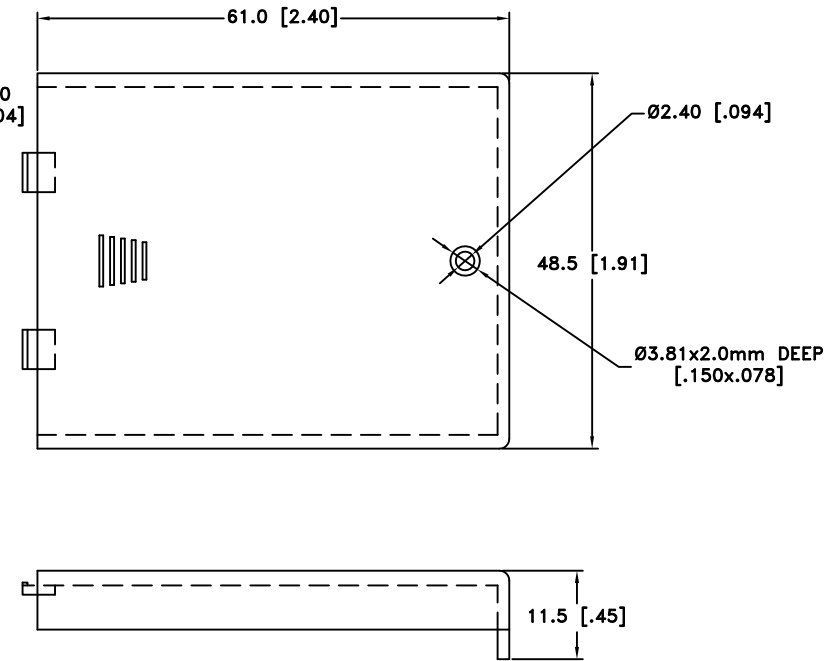
TOP COVER
