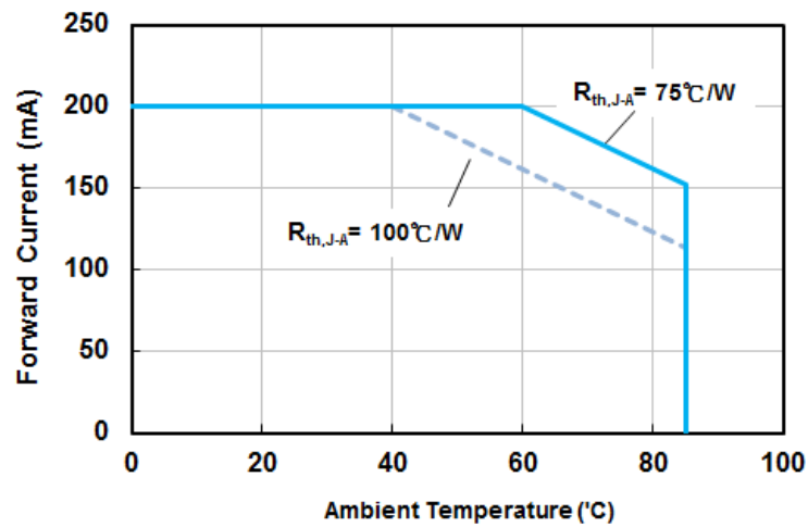
Fig 4. Forward Current derating curve vs Ambient Temperature
