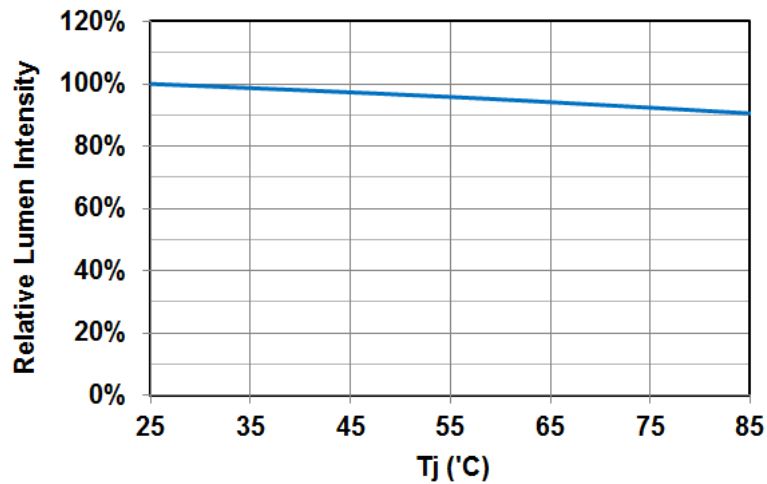
Fig 5. Relative Luminous vs Junction Temperature
