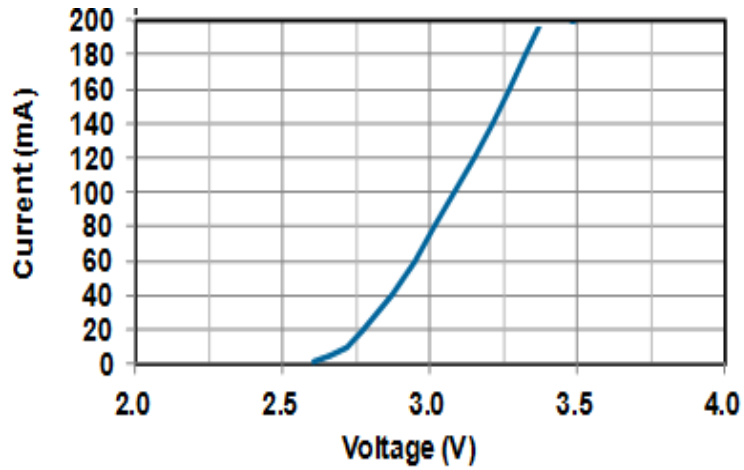
Fig 3. Forward Current vs. Forward Voltage-Curve
