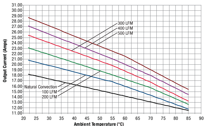
LSM2-T/30-D12 Maximum Current Temperature Derating at Sea Level ( V_{IN} = 12V , Transverse Airflow). No extra ground pads.
