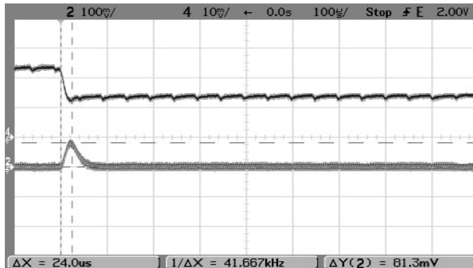
Step Load Transient Response (Vin=14V, Vout=2.5V, Cload=0, Iout=1A to 0.5A, Ta=+25°C.) Trace 2=Vout, 100 mV/div. Trace 4=Iout, 0.5A/div.
