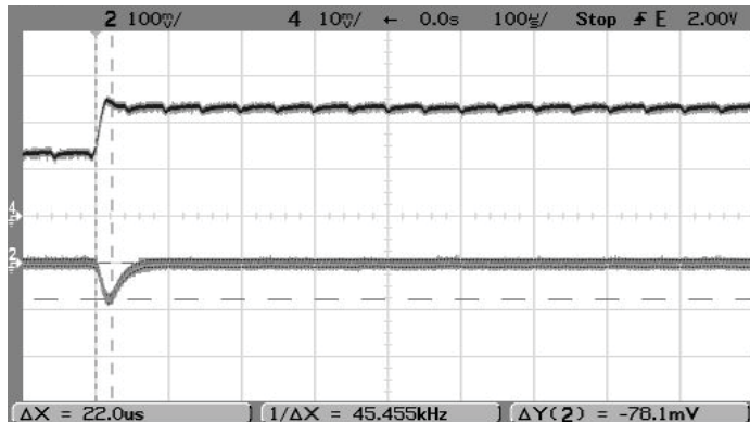
Step Load Transient Response (Vin=14V, Vout=2.5V, Cload=0, Iout=0.5A to 1A, Ta=+25°C.) Trace 2=Vout, 100 mV/div. Trace 4=Iout, 0.5A/div.
