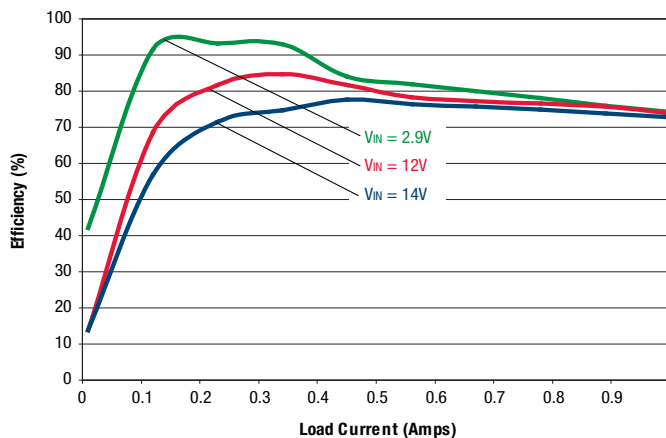
Efficiency vs. Line Voltage and Load Current @Ta = +25 °C (Vout = 1.5V)
