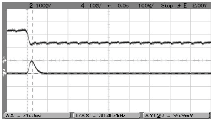
Step Load Transient Response (Vin=4.5V, Vout=3.3V, Cload=0, Iout=1A to 0.5A, Ta=+25°C.) Trace 2=Vout, 100 mV/div. Trace 4=Iout, 0.5A/div.
