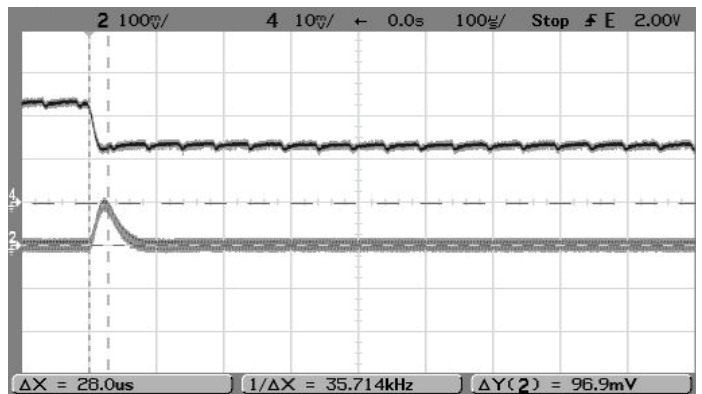
Step Load Transient Response (Vin=12V, Vout=3.3V, Cload=0, Iout=1A to 0.5A, Ta=+25°C.) Trace 2=Vout, 100 mV/div. Trace 4=Iout, 0.5A/div.
