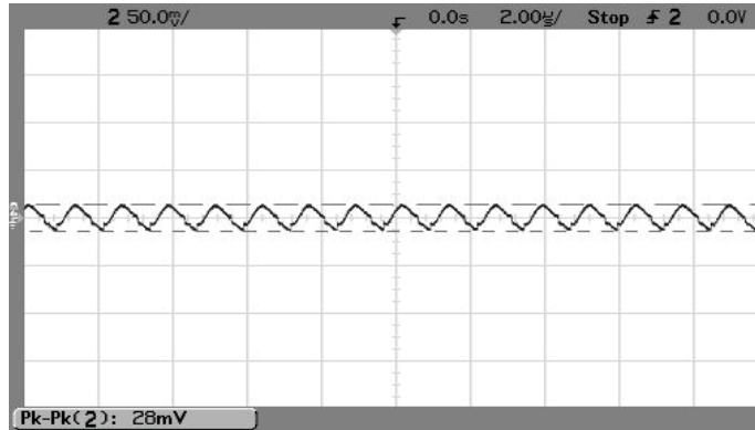
Output Ripple and Noise (Vin=14V, Vout=3.3V, Iout=1A, Cload=0, Ta=+25°C., ScopeBW=100MHz)
