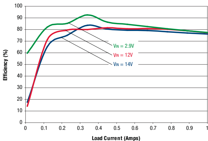
Efficiency vs. Line Voltage and Load Current @Ta = +25 °C (Vout = 1.8V)
