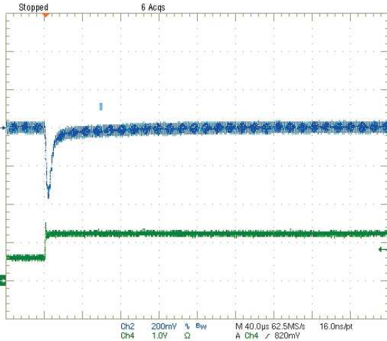
Step Load Transient Response (Vin=12V, Vout=5.0V, Load=0, Iout=3A to 6A) Trace 2=Vout, 200 mV/div. Trace 4=Iout, 5A/div.
