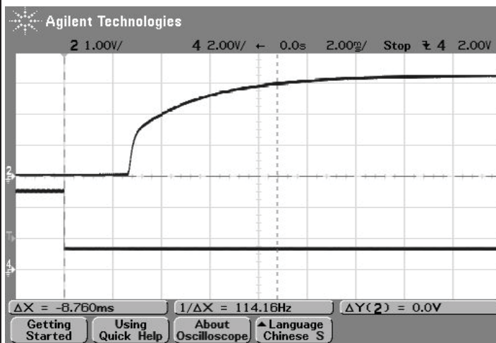
On/Off Enable Delay (Vin=48V, Vout=nom., Iout=25A, Cload=10uF, Ta=+25° C., ScopeBW=20Mhz, Trace 2=Vout, Trace 4=Enable.)
