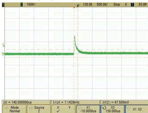
Step Load Transient Response (Slew=1A / \mu Sec., Vin=48V., Cload=0, Iout=15A to 22.5A)
