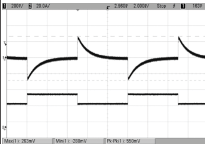
Step Load Transient Response (Vin=48V, Vout=nom, Load= 1uF || 10uF, Iout=50 to 75 to 50% of full load, Ta=+25°C) Ch1=Vout, Ch2=Iout.
