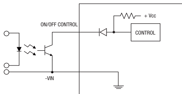
Figure 5. Driving the Logic On/Off Control Pin
