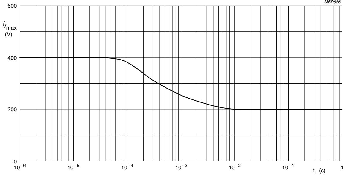
Fig. 13 Pulse on a regular basis; maximum permissible peak pulse voltage ( \hat{V}_{max} ) as a function of pulse duration ( t_i ).
