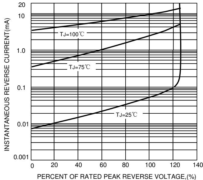
FIG.5-TYPICAL REVER CHARACTERISTICS
