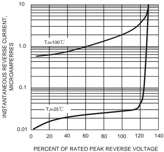
FIG.3-TYPIACL REVERSE CHARACTERISTICS
