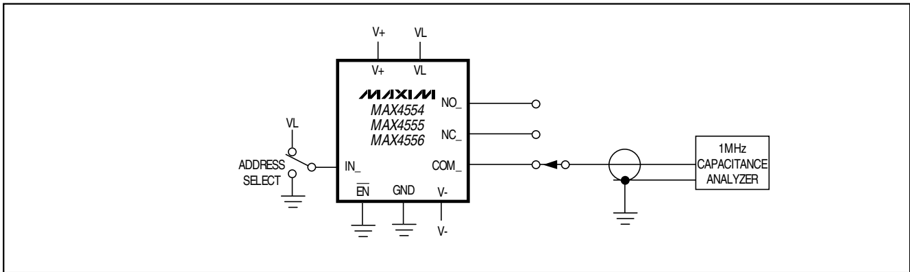
Figure 14. COM 1 , NO 1 , NC 1 Capacitance
