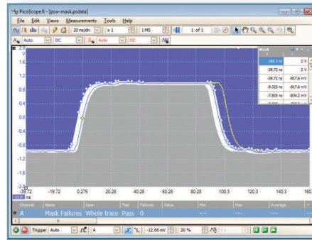
Mask limit testing
