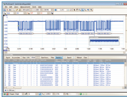
Serial data decoding
