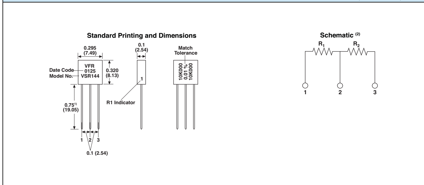
FIGURE 2 - MODEL VSR144 STANDARD PRINTING AND DIMENSIONS in inches (millimeters)
