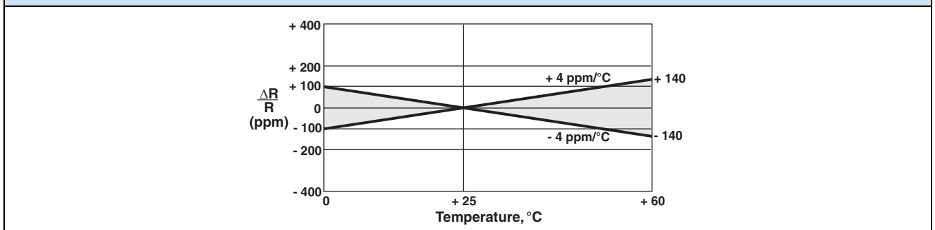
FIGURE 1 - TEMPERATURE COEFFICIENT OF RESISTANCE
