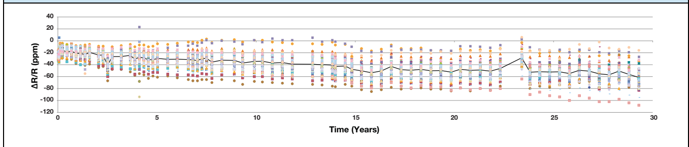
FIGURE 5 - LONG-TERM STABILITY OVER 29 YEARS (0.1W AT 70°C, 50 SAMPLES RCK02, 10KΩ)
