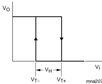
Fig 9. Transfer characteristic
