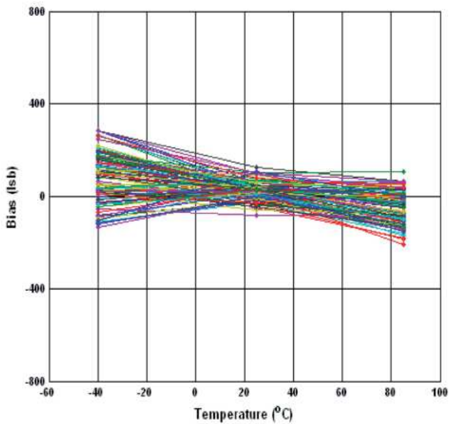
Figure 5.21 Digital Bias vs Temperature
