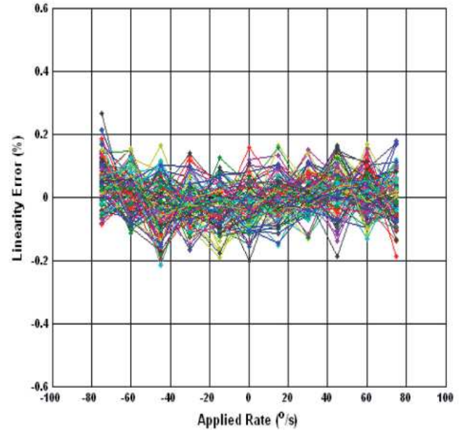
Figure 5.28 Digital Output Linearity Error vs Applied Rate at +85°C
