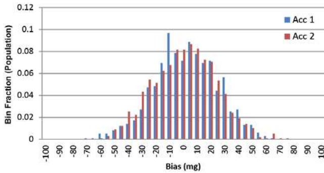
Figure 5.13 Acceleration Bias Distribution at 25°C (±10g)
