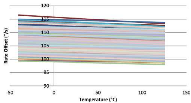
Figure 5.9 CBIT %s vs Temperature (±300°/s)
