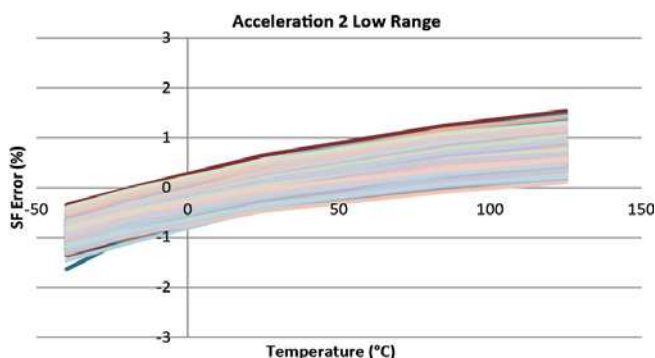
Figure 5.22 Accelerometer X SF Error vs Temperature ( \pm 2.5g )
