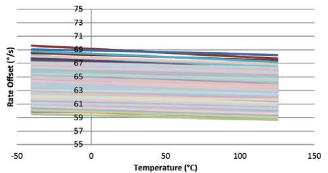
Figure 5.10 CBIT %s vs Temperature (±150°/s)
