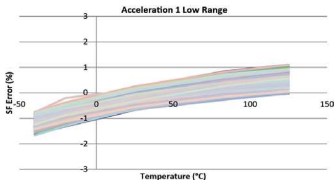
Figure 5.20 Accelerometer Y SF Error vs Temperature ( \pm 2.5g )
