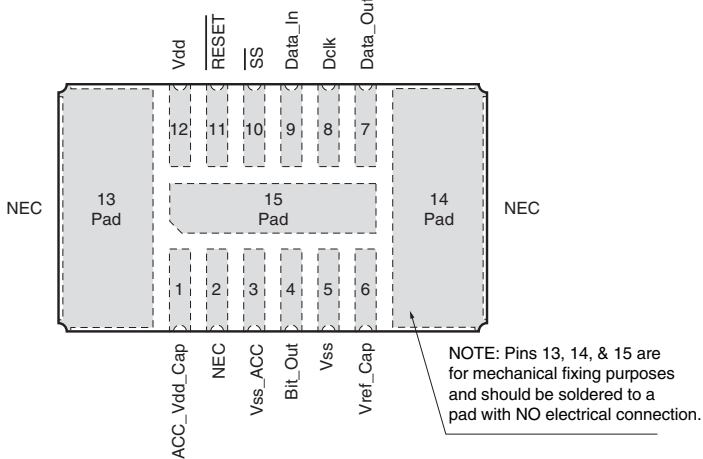
Figure 7.1 Pinout (Top View)
