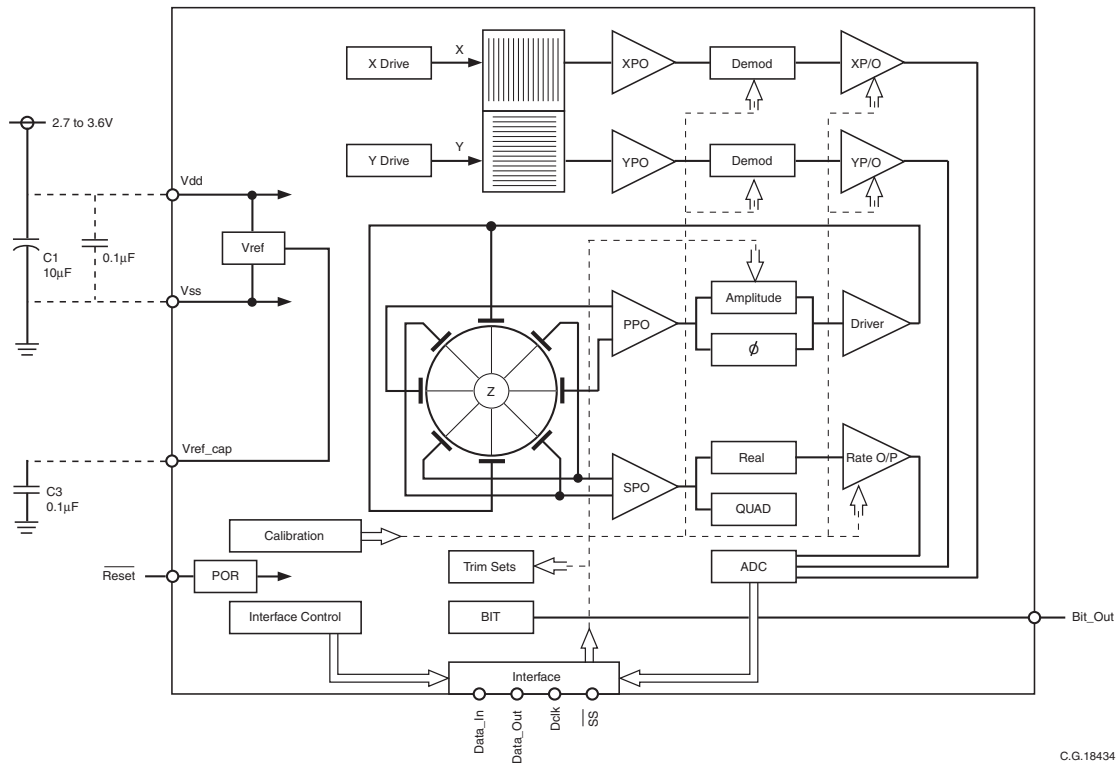
Figure 1.1 CMS300 Functional Block Diagram
