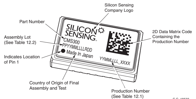
Figure 12.1 Part Marking
