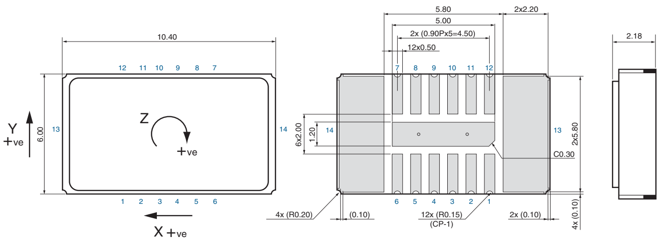
Figure 1.2 CMS300 Overall Dimensions
