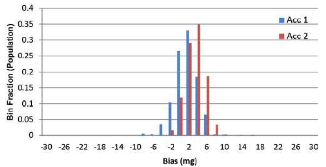
Figure 5.14 Acceleration Bias Distribution at 25°C (±2.5g)
