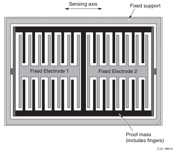
Figure 14.5(a) Schematic of Accelerometer Structure
