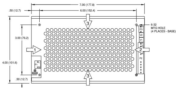
OPTIONAL COVER
