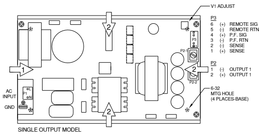
STANDARD CHASSIS
