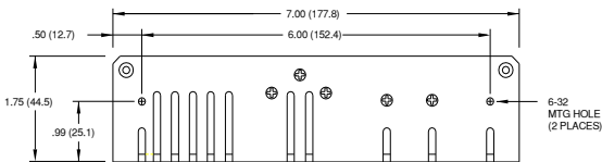
OPTIONAL COVER
