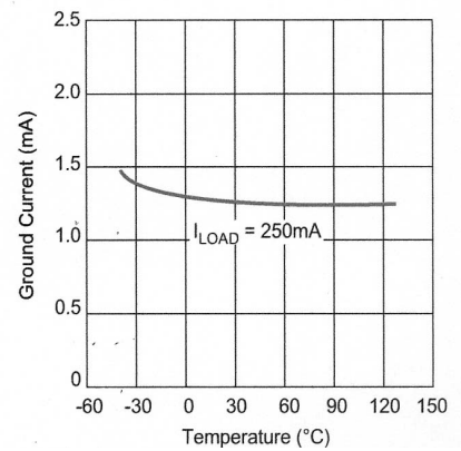
Figure 6. LM29150 Ground Current vs. Temperature
