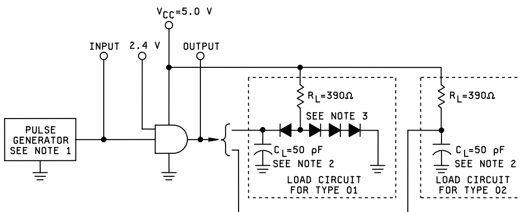
TEST CIRCUIT
