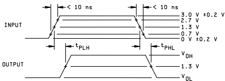
VOLTAGE WAVEFORMS
