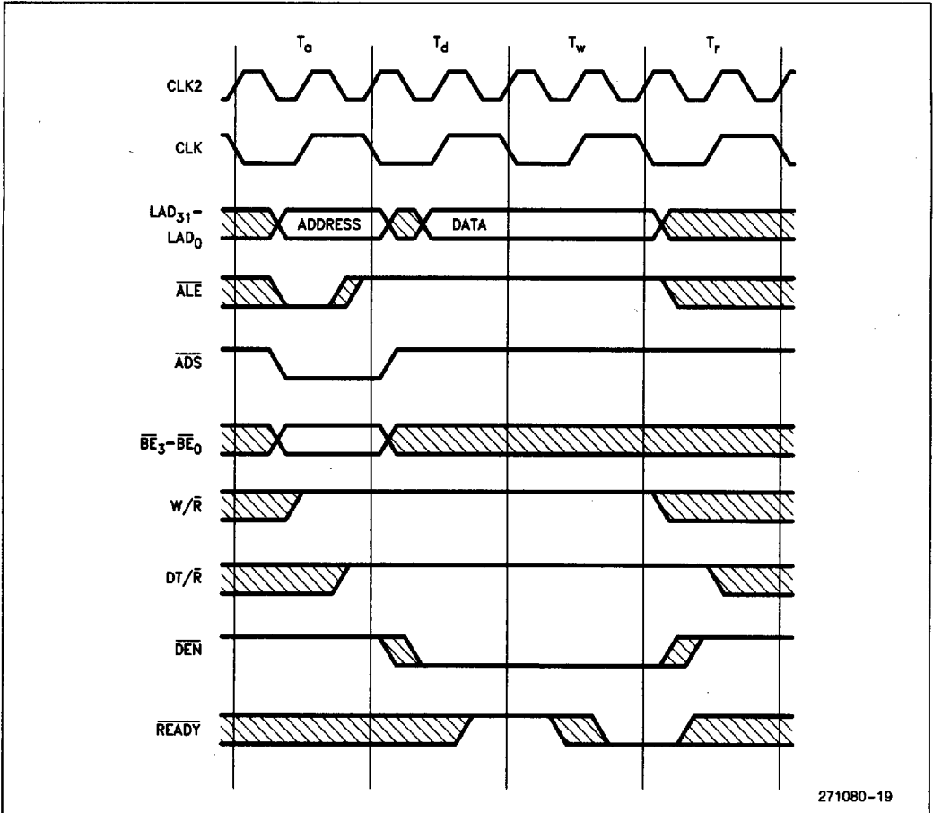
Figure 26. Write Transaction with One Wait State
