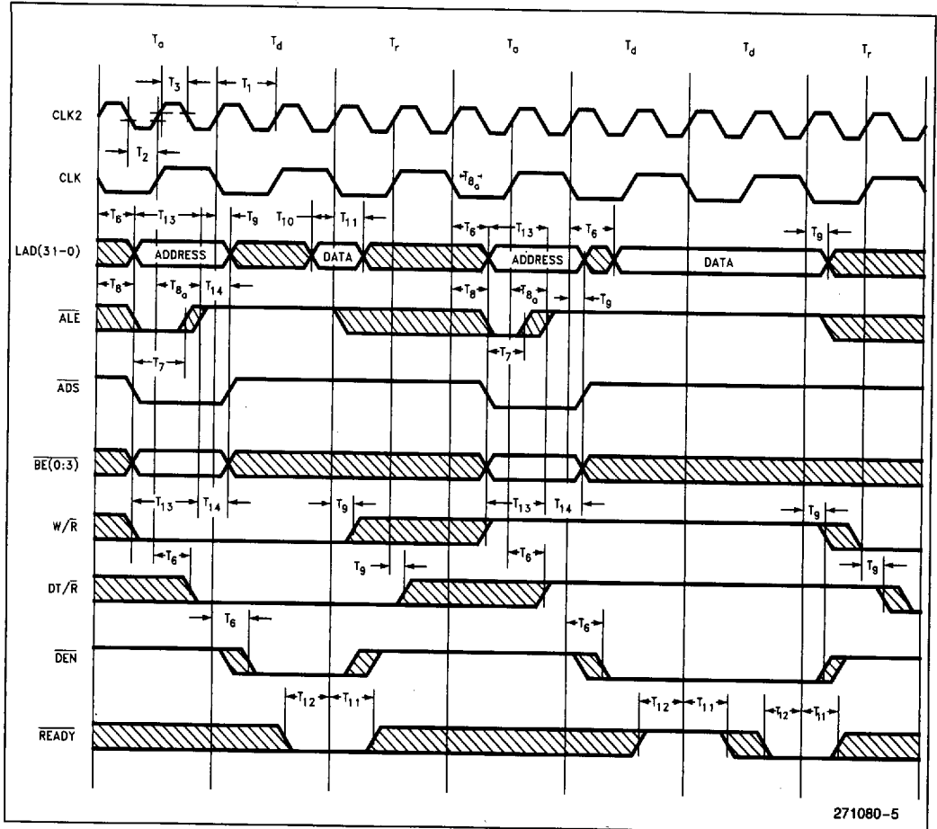
Figure 13. Timing Relationship of L-Bus Signals
