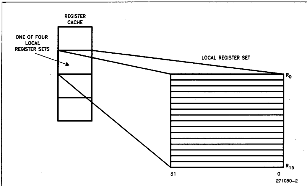
Figure 4. Multiple Register Sets Are Stored On-Chip
