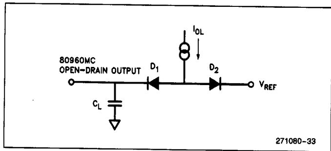
Figure 11. Test Load Circuit for Open-Drain Output Pins
