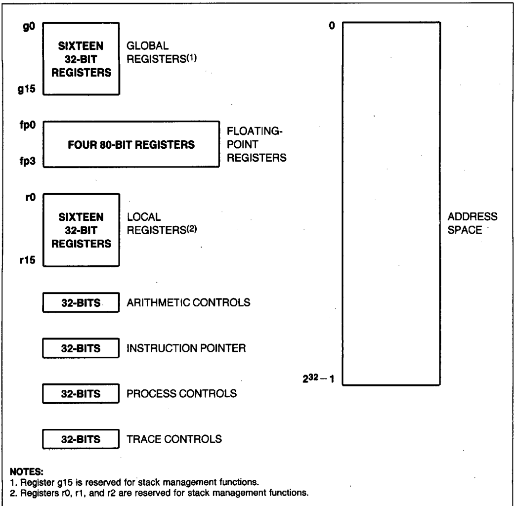
Figure 2. Register Set
