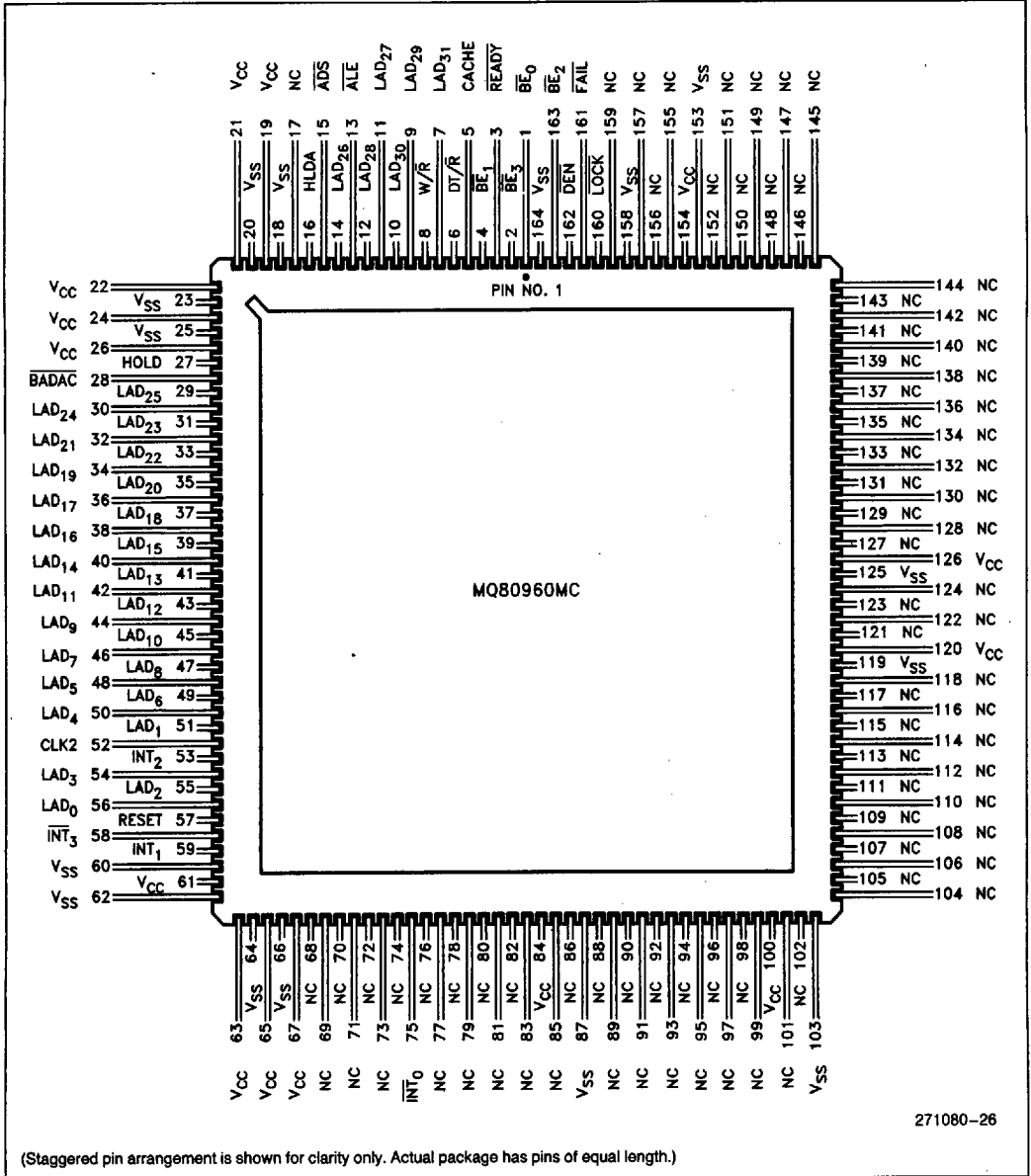
Figure 20. MQ80960MC Pinout—View from Top of Package
