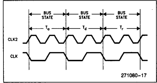
Figure 24. System and Processor Clock Relationship
