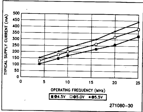
Figure 8. Typical Current vs Frequency
