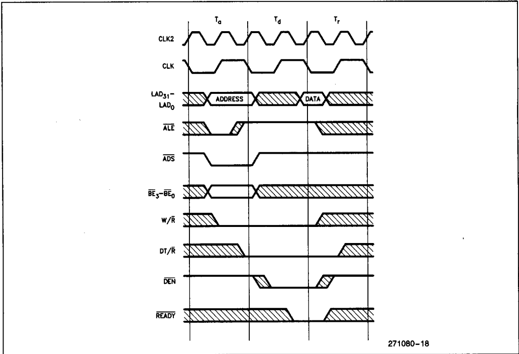
Figure 25. Read Transaction
