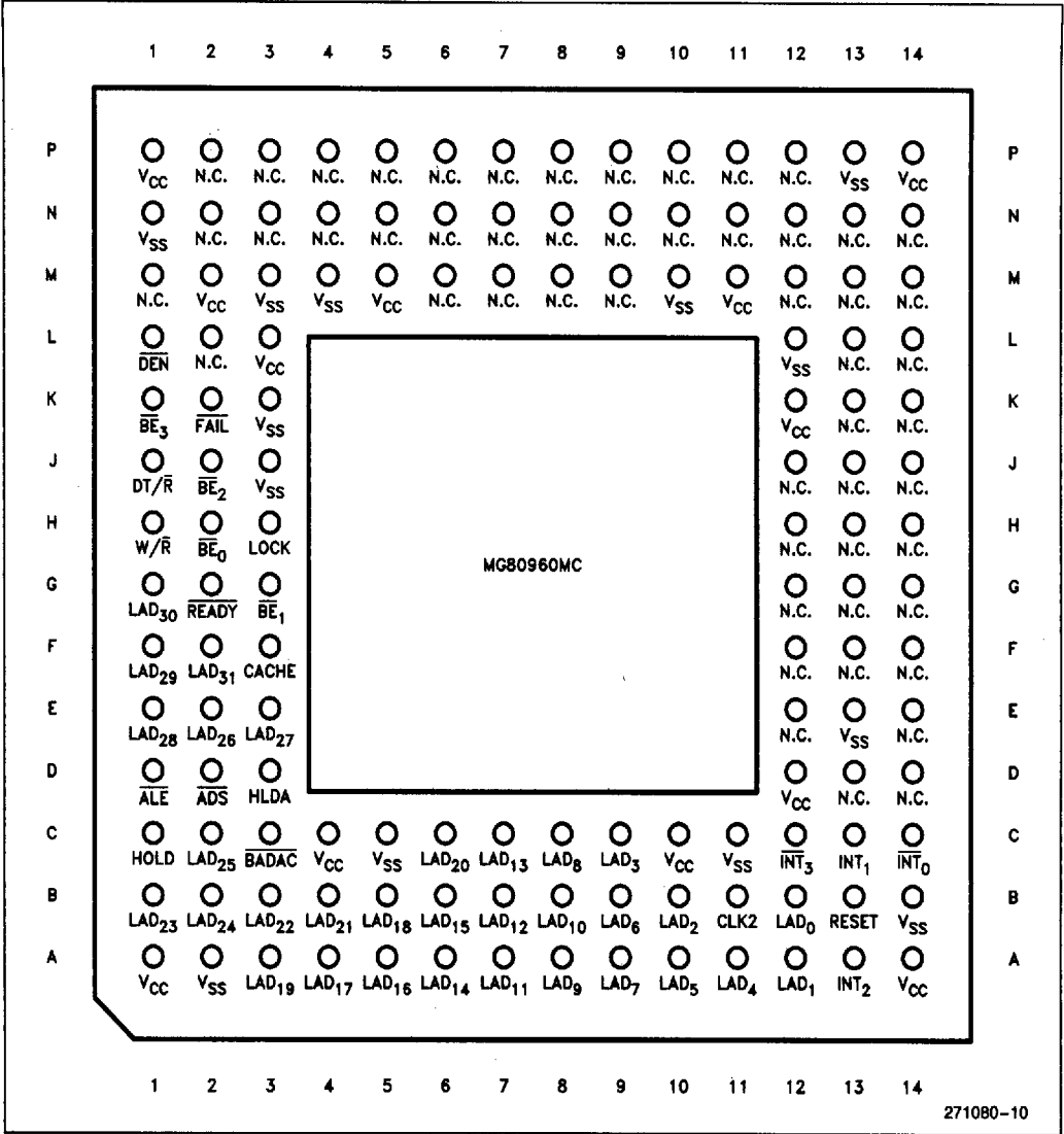
Figure 19. MG80960MC Pinout—View from Bottom (Pins Facing Up)
