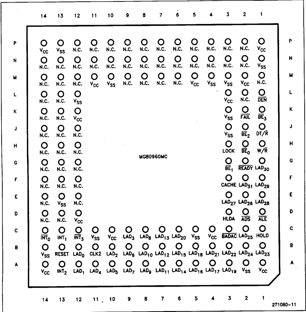
Figure 18. MG80960MC Pinout—View from Top (Pins Facing Down)
