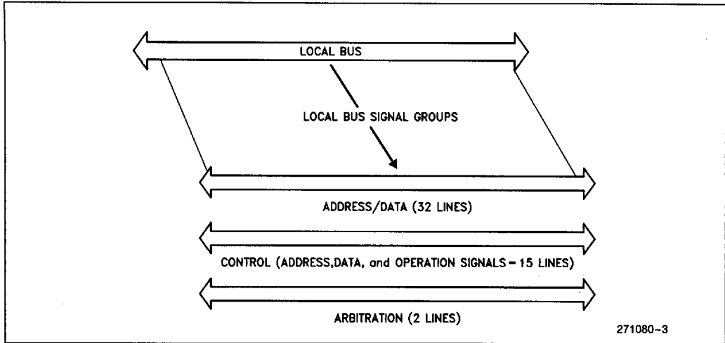
Figure 5. Local Bus Signal Groups
