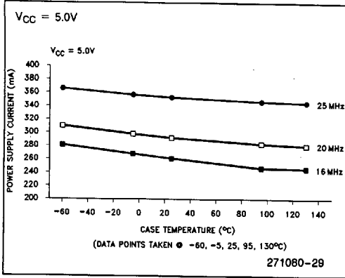
Figure 7. Typical Supply Current ( I_{CC} )
