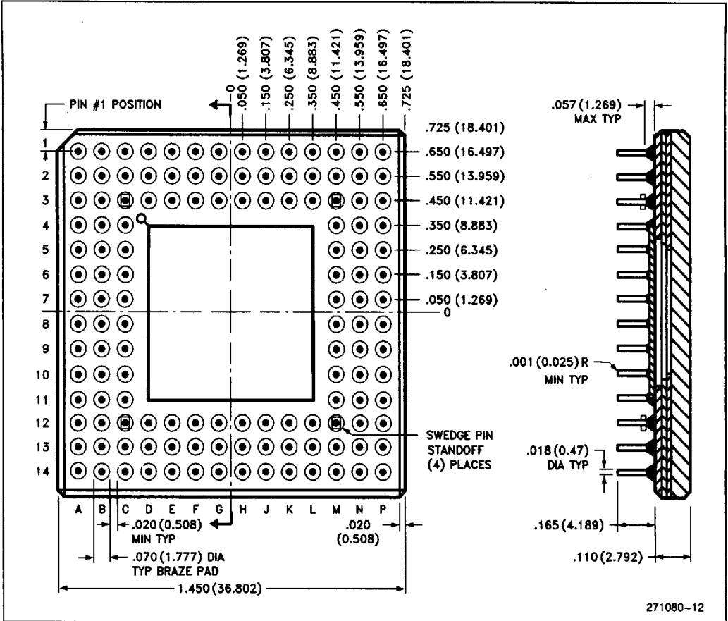
Figure 21. A 132-Lead Pin-Grid Array (PGA) Used to Package the MG80960MC
