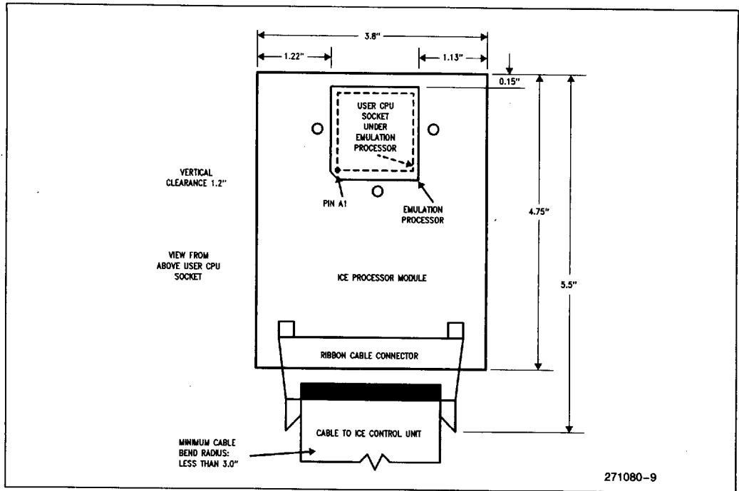
Figure 17. ICE-960MC Lateral Clearance Requirements
