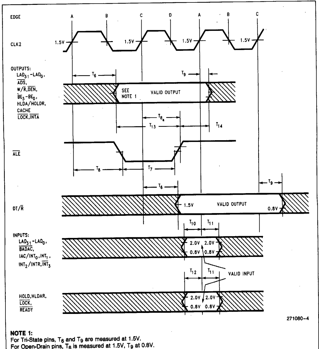
Figure 12. Drive Levels and Timing Relationships for 80960MC Signals
