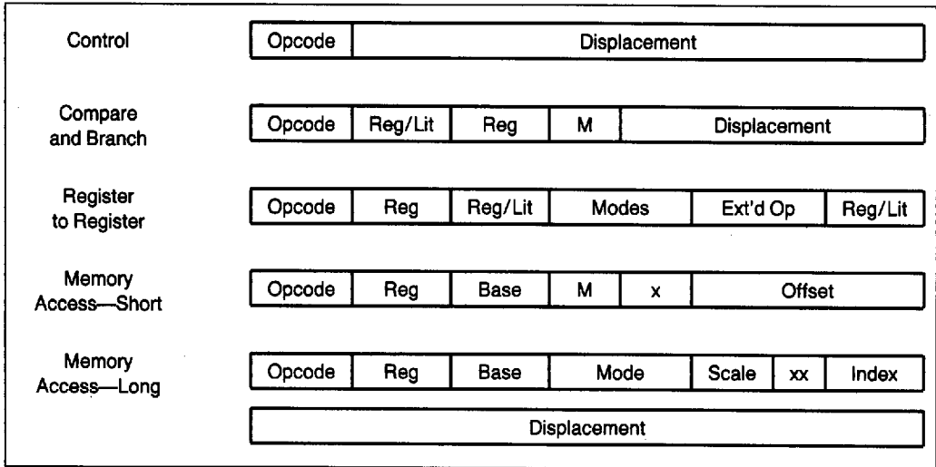
Figure 3. Instruction Formats
