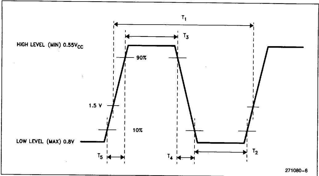
Figure 14. Processor Clock Pulse (CLK2)
