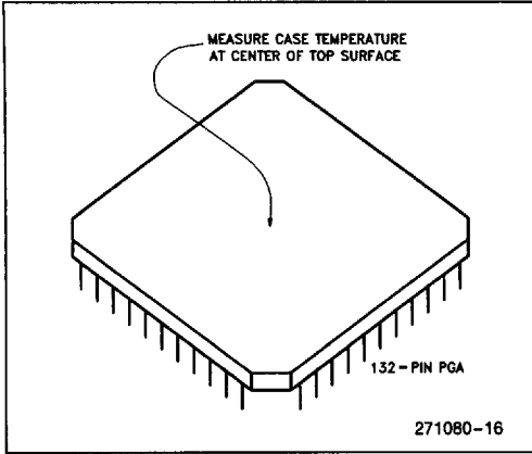
Figure 23. Measuring MG80960MC PGA Case Temperature ( T_C )
