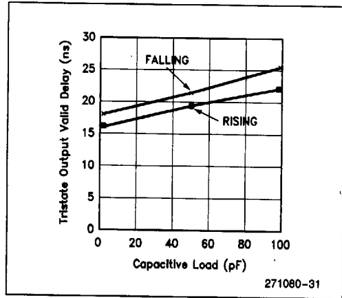
Figure 9. Capacitive Derating Curve
