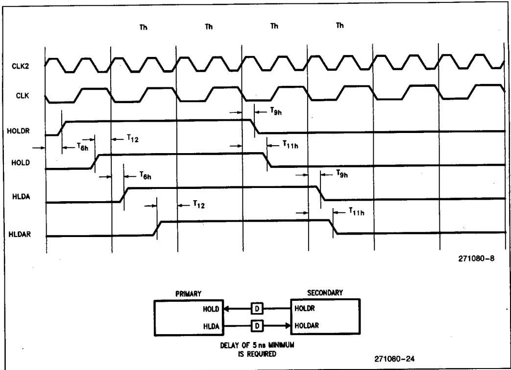
Figure 16. Hold Timing
