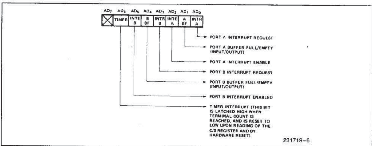
Figure 6. Status Register Bit Assignment
