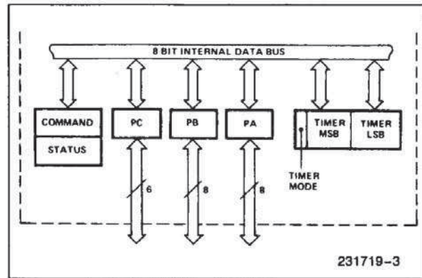
Figure 3. 8155H/8156H Internal Registers
