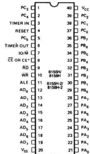
Figure 2. Pin Configuration
