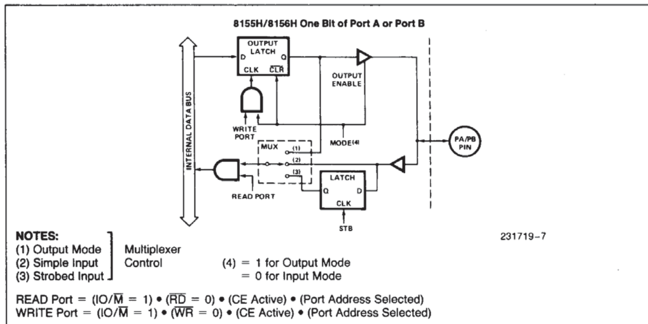
Figure 8. 8155H/8156H Port Functions
