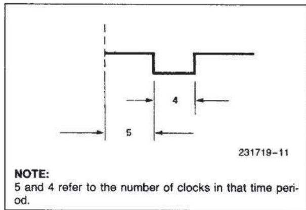
Figure 12. Asymmetrical Square-Wave Output Resulting from Count of 9
