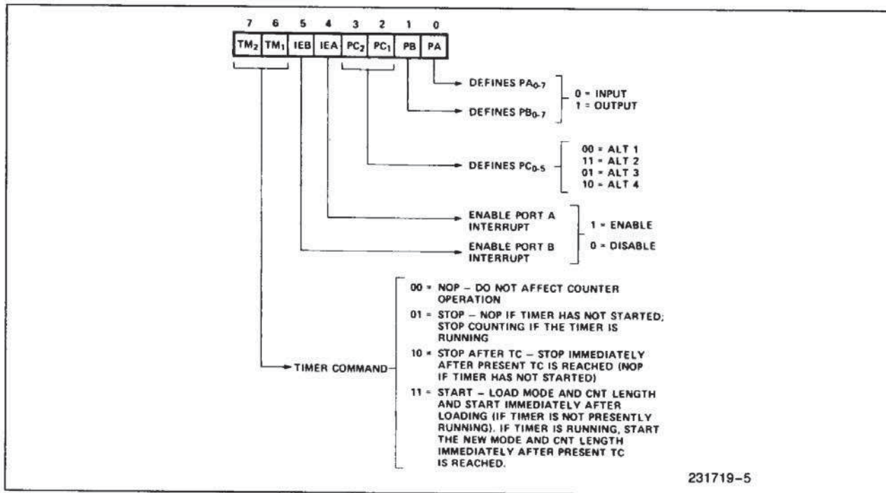
Figure 5. Command Register Bit Assignment
