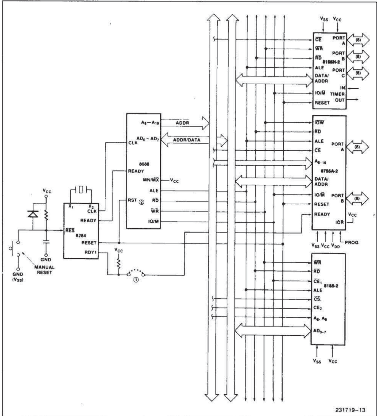
Figure 13b. 8088 Five Chip System Configuration
