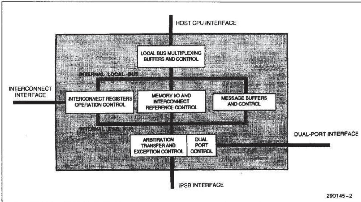
Figure 3-1. MPC Bus Interfaces
