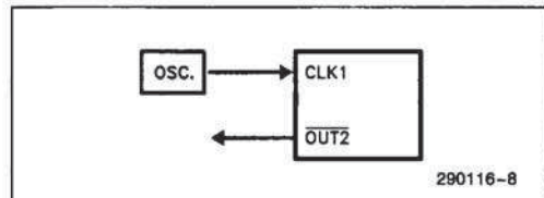
Figure 8. External Clock
