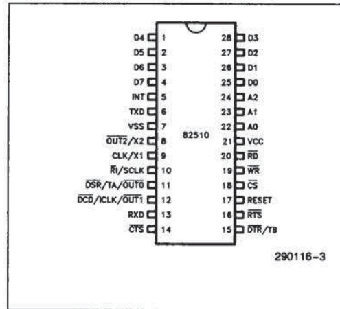
Figure 3. DIP Pinout
