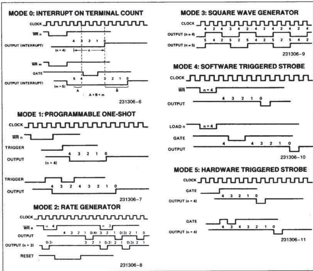
Figure 7. 8253 Timing Diagrams
