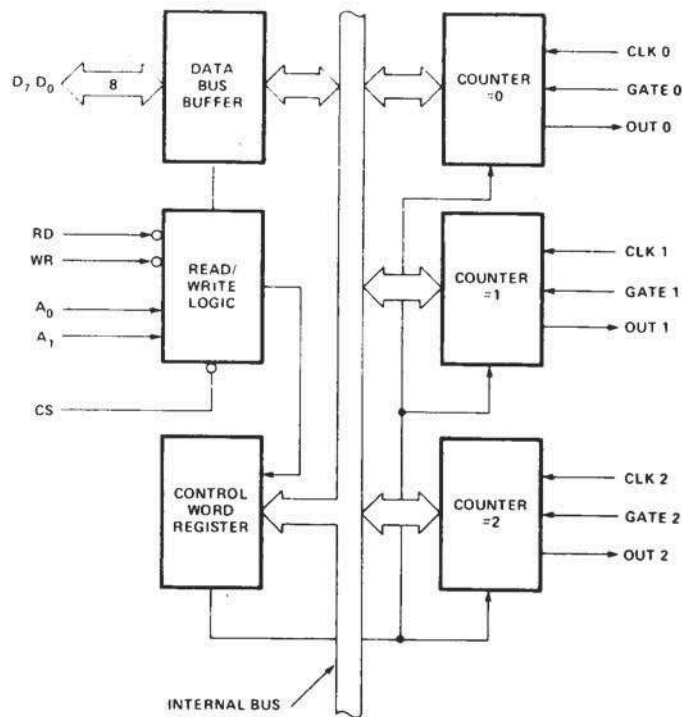
Figure 1. Block Diagram
