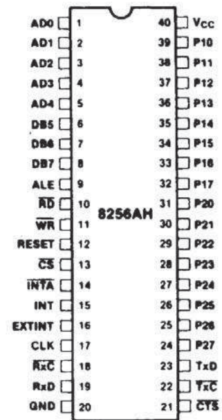
Figure 2. MUART Pin Configuration
