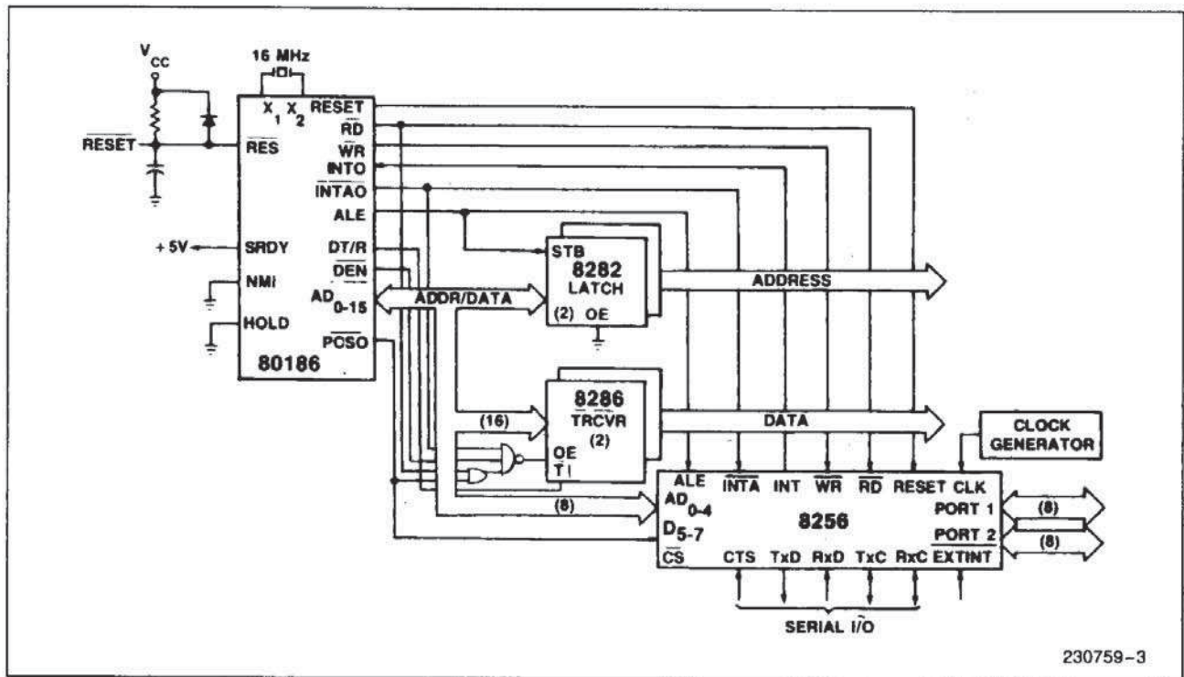
Figure 3. 80186/8256 Interface
