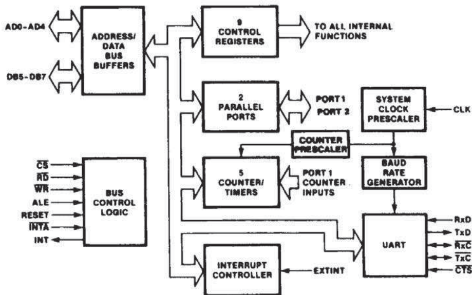
Figure 1. MUART Block Diagram
