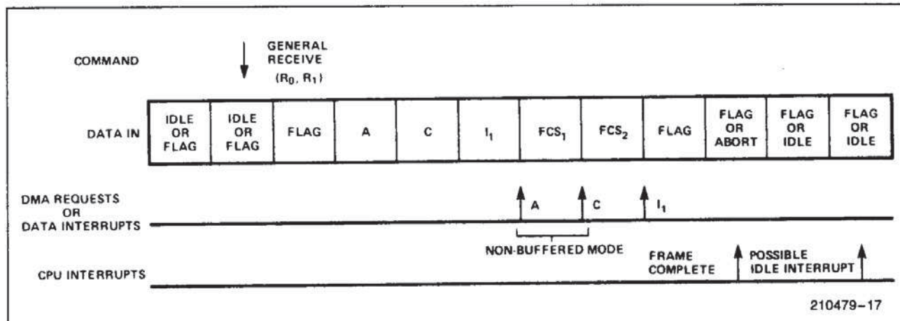
Figure 16. Typical Frame Reception
