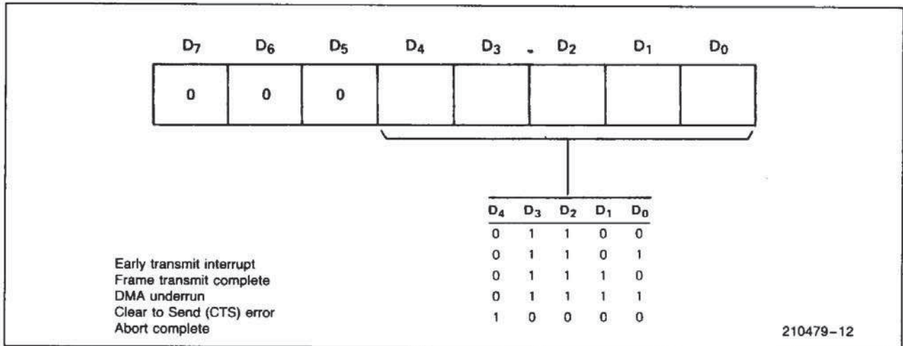
Figure 12. Tx Interrupt Result Byte Format
