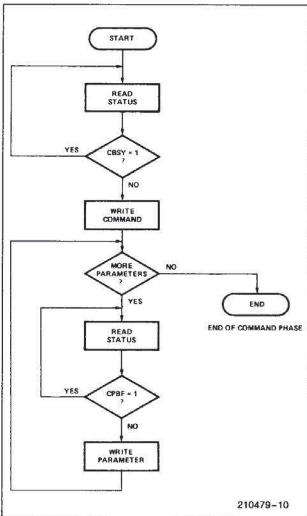
Figure 10. Command Phase Flowchart
