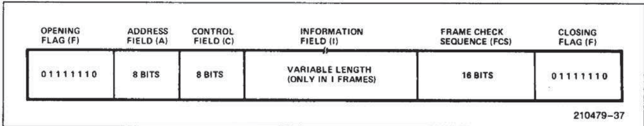
Figure 4. Frame Format
