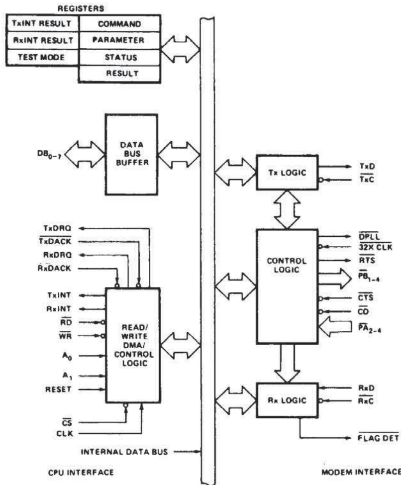
Figure 1. Block Diagram
