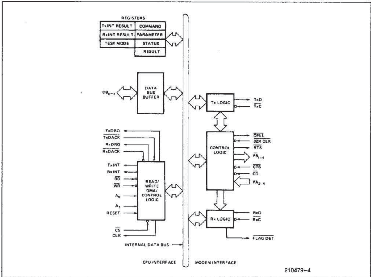
Figure 6. 8273 Block Diagram Showing Control Logic Functions
