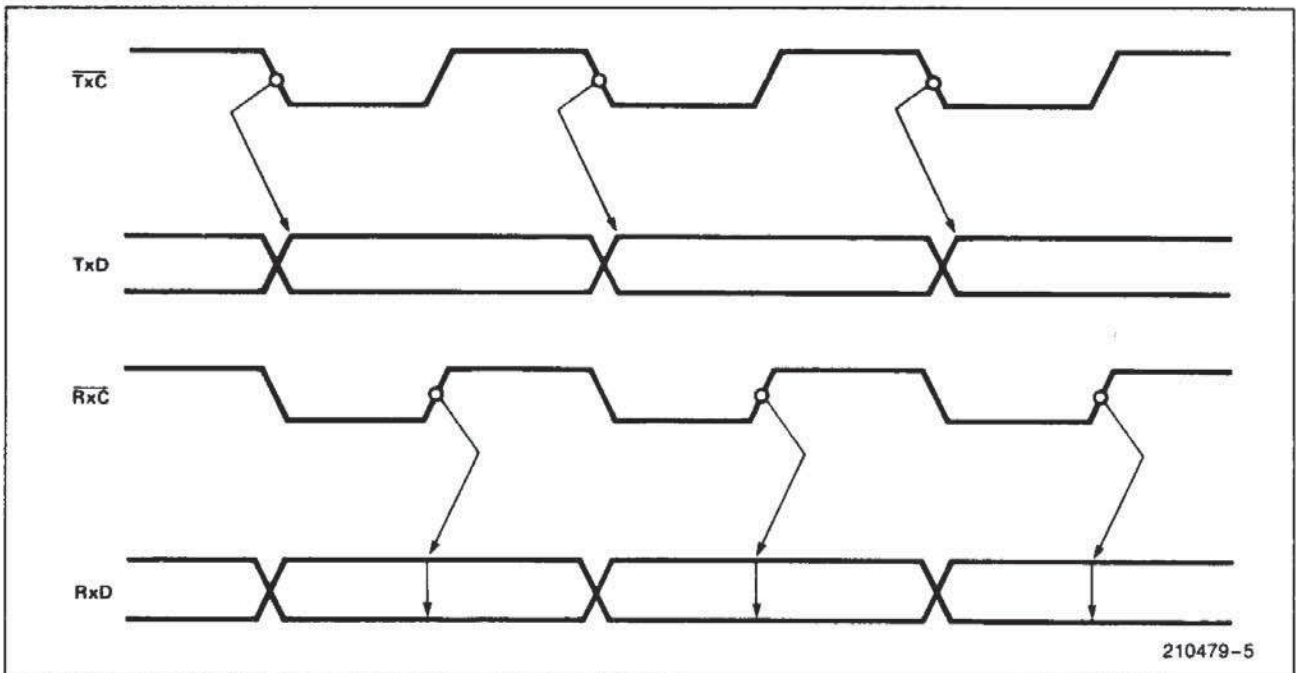
Figure 7. Transmit/Receive Timing
