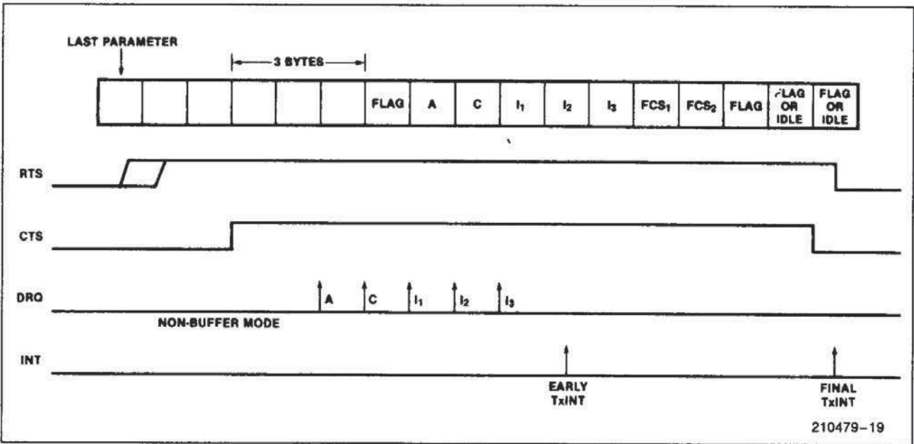
Figure 17b. Typical Frame Transmission, Non-Buffered Mode
