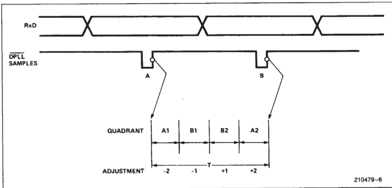
Figure 8. DPLL Sample Timing
