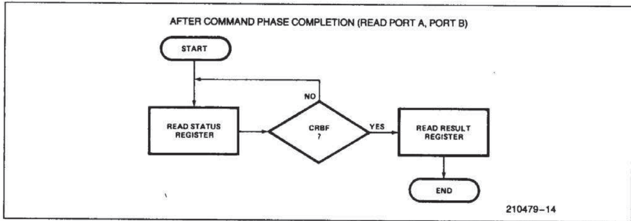
Figure 14. (Rx Interrupt Service)
