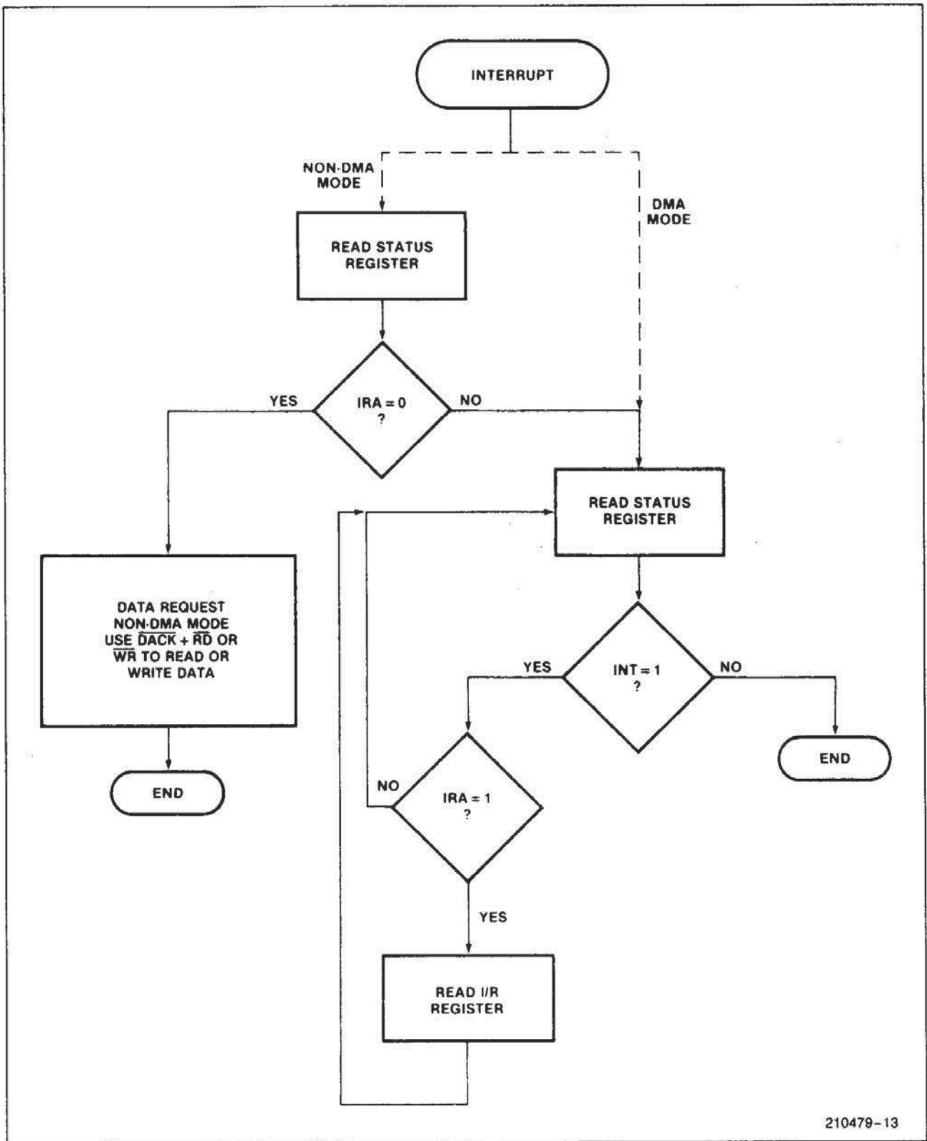
Figure 13. Result Phase Flowchart—Interrupt Results
