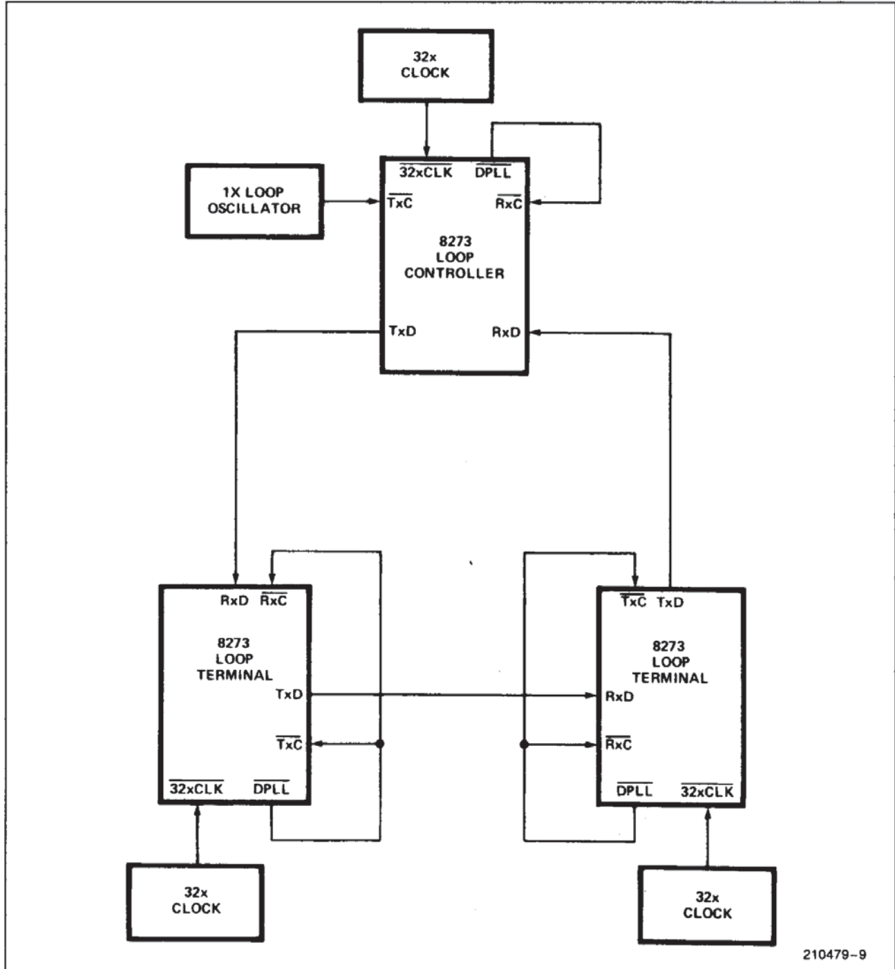
Figure 9. SDLC Loop Application
