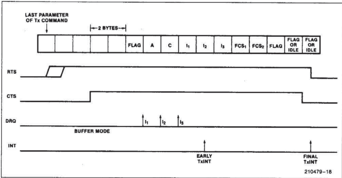
Figure 17a. Typical Frame Transmission, Buffered Mode
