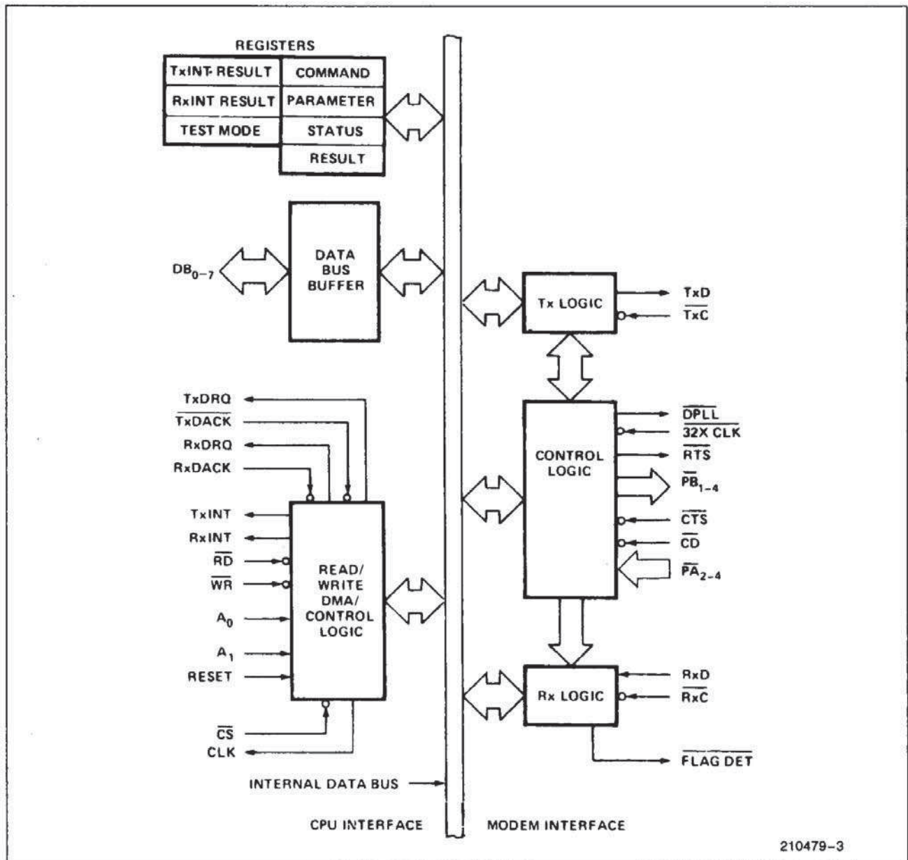
Figure 5. 8273 Block Diagram Showing CPU Interface Functions
