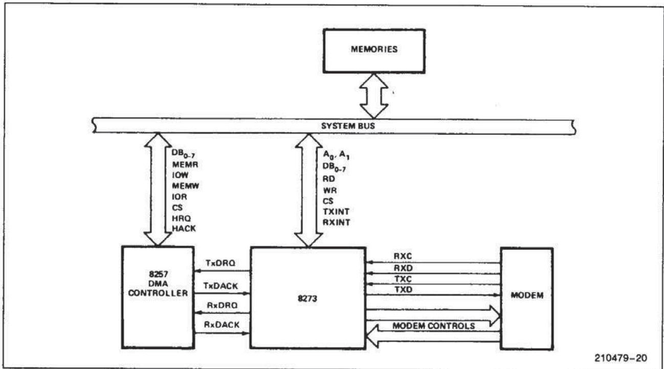
Figure 18. 8273 System Diagram
