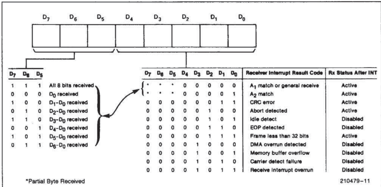
Figure 11. Rx Interrupt Result Byte Format
