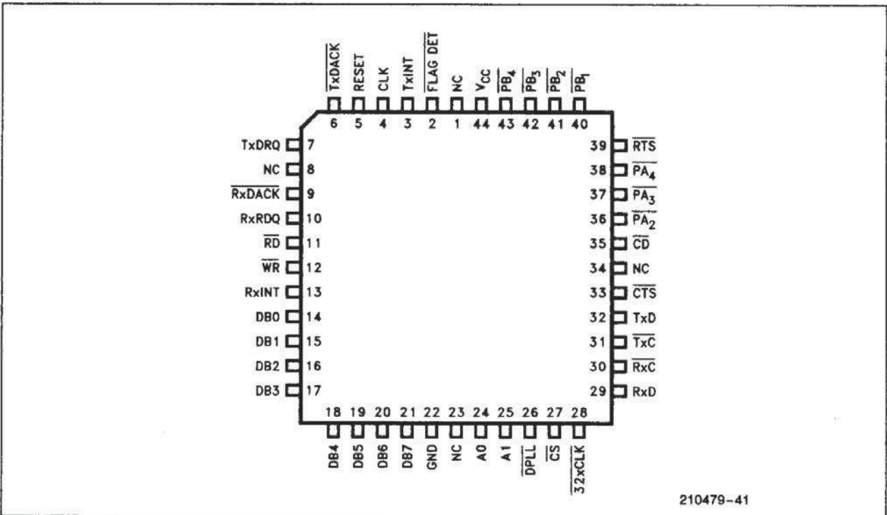
Figure 3. 8273 Pin Configuration (PLCC)
