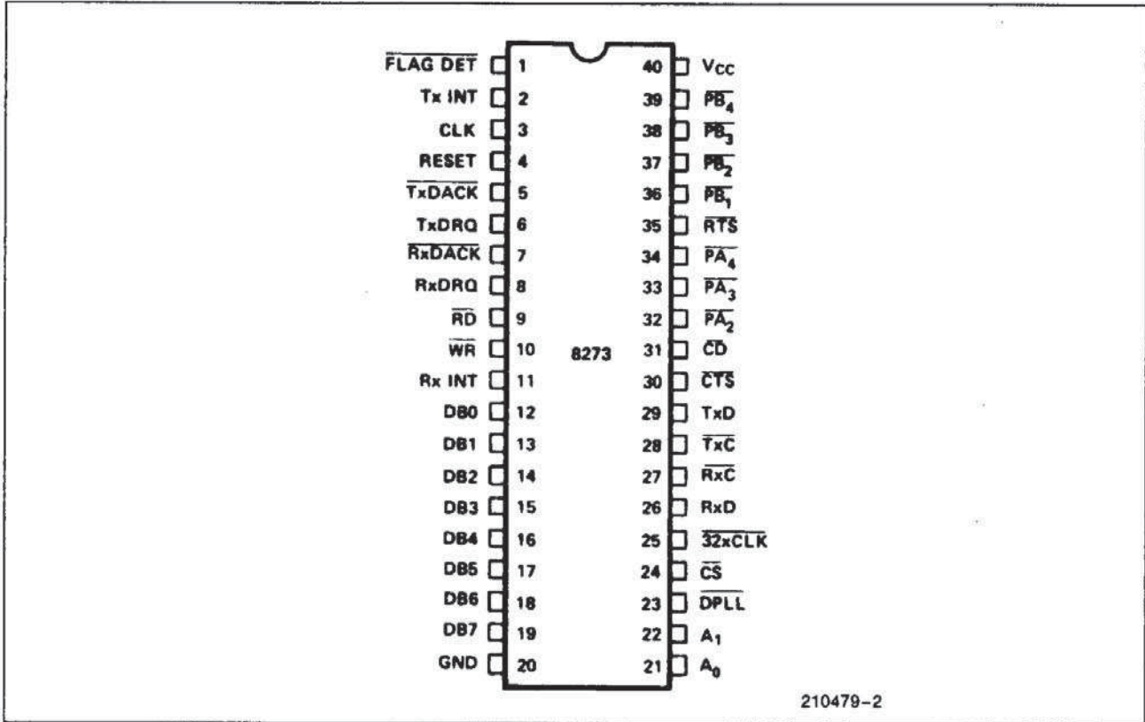
Figure 2. Configuration (PDIP)
