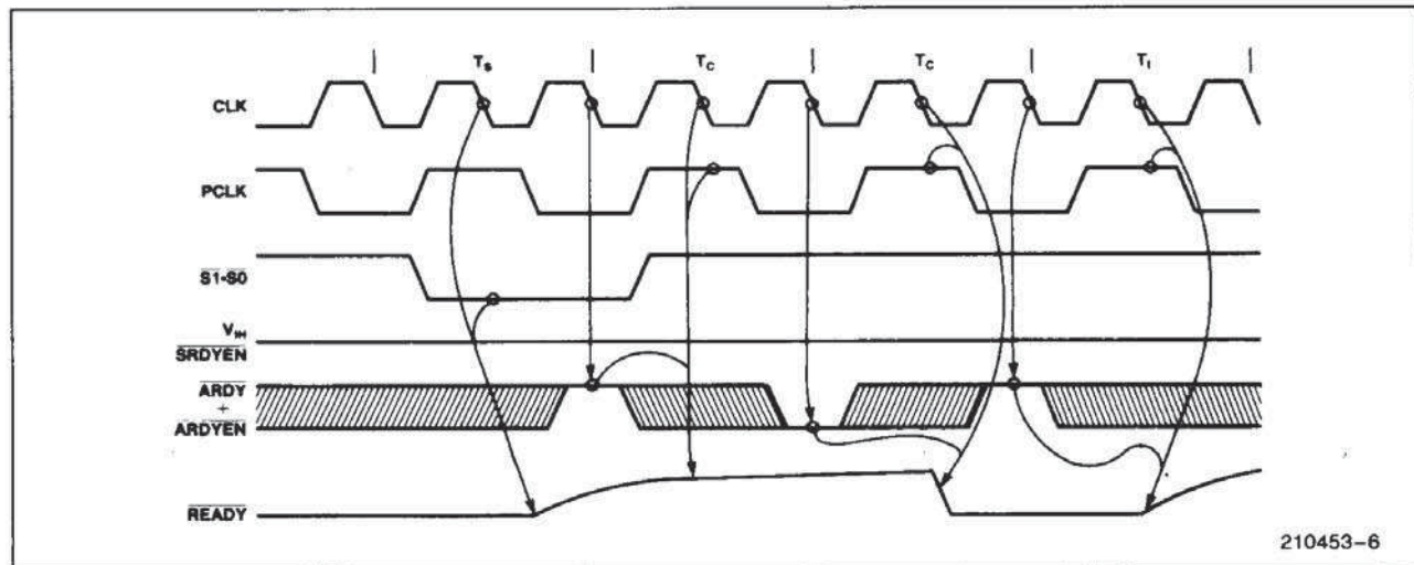
Figure 7. Asynchronous Ready Operation
