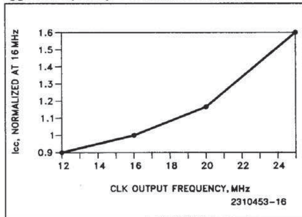
I CC vs Frequency @ Nominal Conditions
