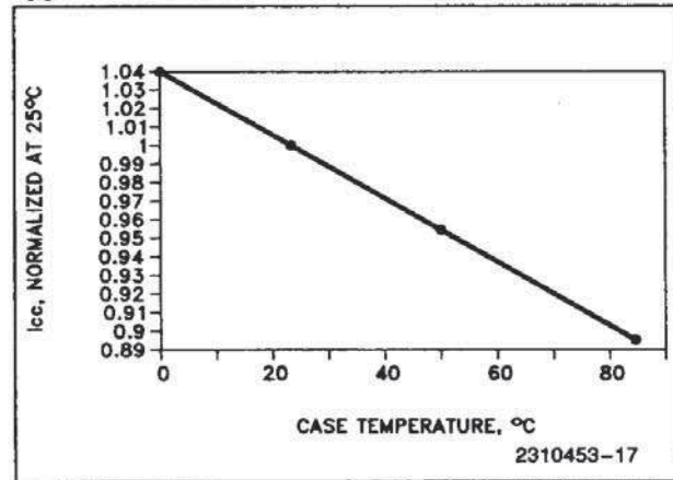
I CC vs Case Temperature @ 25 MHz
