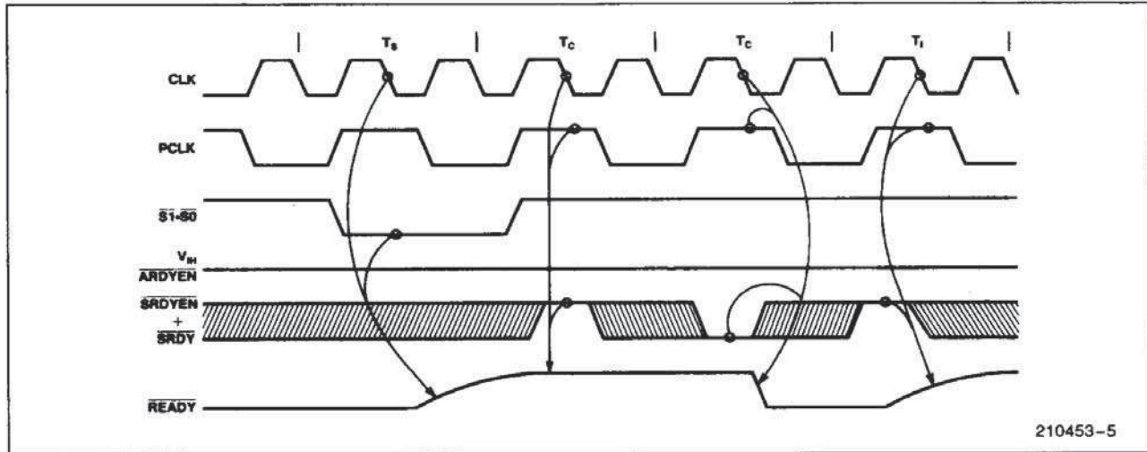
Figure 6. Synchronous Ready Operation
