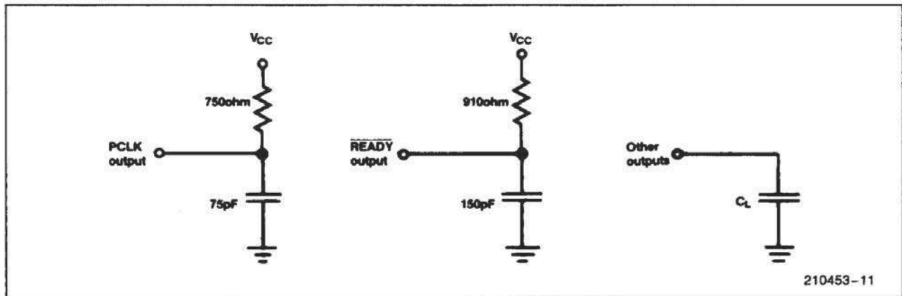
Note 13. AC Test Loading on Outputs
