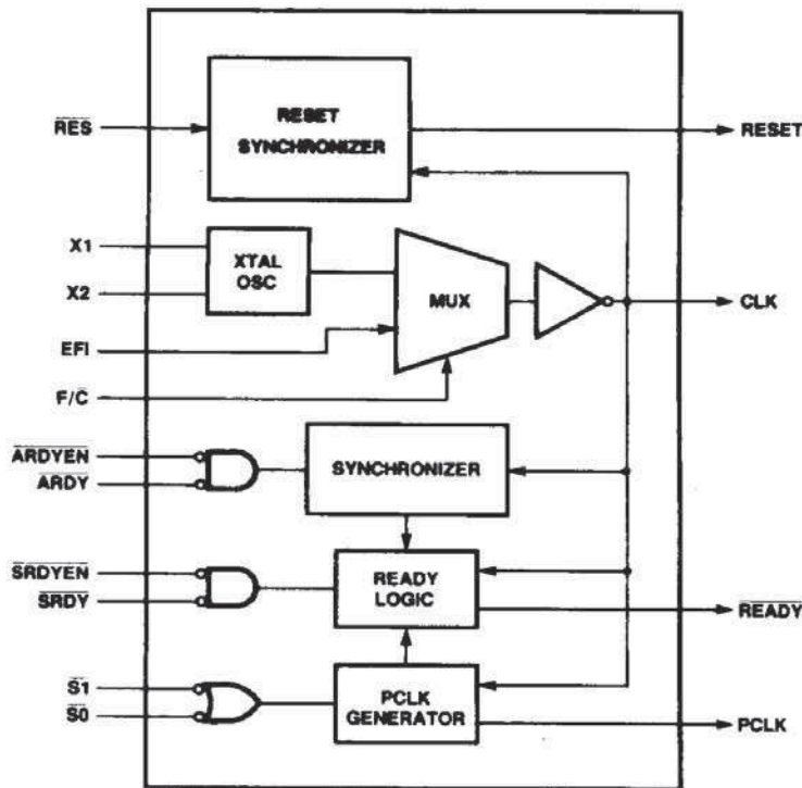
Figure 1. 82C284 Block Diagram
